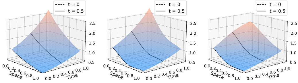
FIG 5. Functions u_{\text{model}} (left), u^* (middle), and regularized PINN estimator with n = 10^3 (right).
