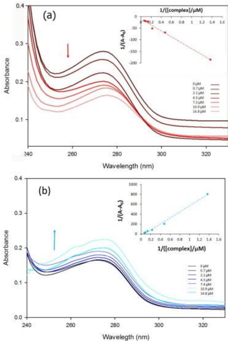
Fig. 10. The change of electronic absorption spectra of HSA upon addition of various amounts of (a) \text{MoO}_2\text{L}(\text{LH}_2)^1 and (b) \text{MoO}_2\text{L}(\text{LH}_2)^2 complexes.
