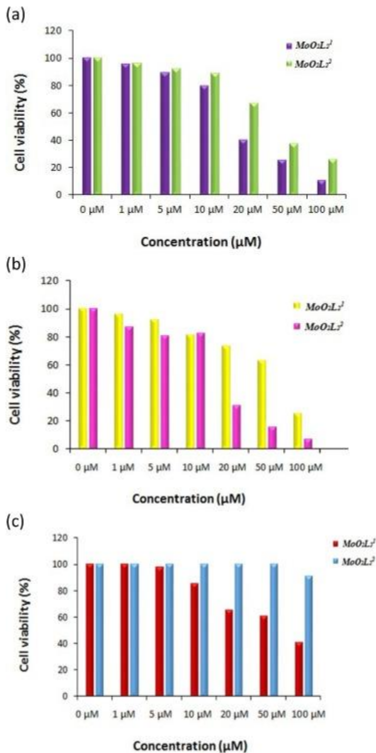
Fig. 15. The viability percentage of (a) MCF-7, (b) HeLa cancer cells and (c) normal fibroblast cells after treatment with different concentrations of Mo(VI) complexes for 48 h.
