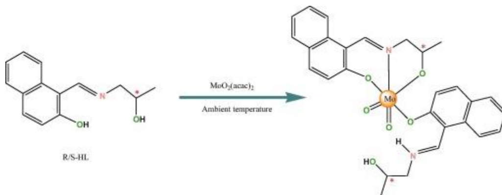
Scheme 1. Synthesis of Mo(VI) complex.
