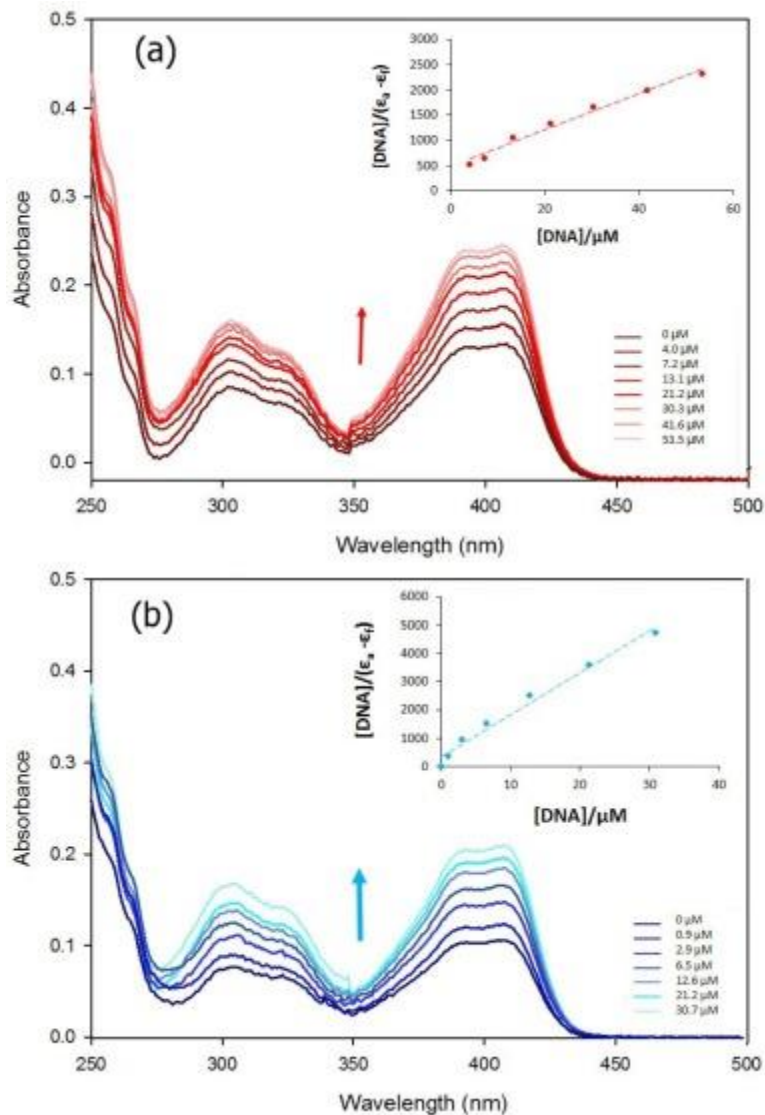
Fig. 6. The change of electronic absorption spectra of (a) \text{MoO}_2\text{L}(\text{LH}_2)^1 and (b) \text{MoO}_2\text{L}(\text{LH}_2)^2 complexes ( 1 \times 10^{-5} M) upon addition various amounts of FS-DNA ( 1 \times 10^{-4} M).
