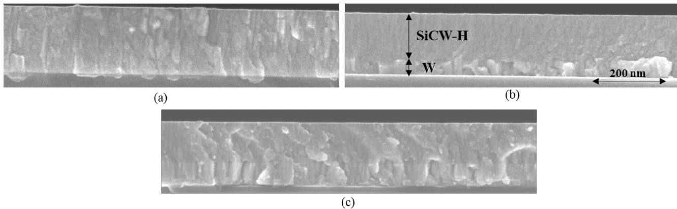
Figure 6: Cross-section SEM images of samples deposited with (a) 1%, (b) 8% and (c) 20% of TMS in the Ar/TMS plasma for the WSiC:H top layer
