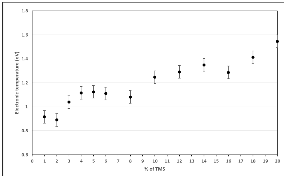
Figure 2: Evolution of the electron temperature of an Ar + W + TMS RF reactive MW PVD plasma with TMS precursor content
