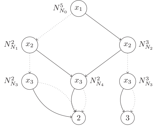
Figure 10: An \text{ADD} representation equivalent to \alpha . The domain of all variables is \{0, 1\} . Every dotted (resp. plain) arc a corresponds to the value v(a) = 0 (resp. v(a) = 1 ).
