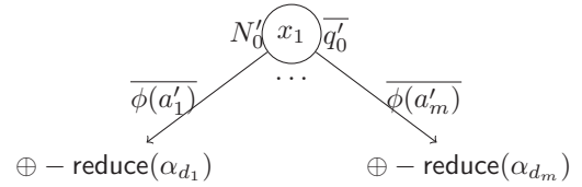
Figure 4: \oplus -reduction of the e-SLDD \alpha' .
