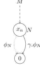
Figure 7: min -normalization of \beta .
