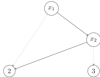
Figure 11: A reduced \text{ADD} representation equivalent to \alpha . The domain of all variables is \{0, 1\} . Every dotted (resp. plain) arc a corresponds to the value v(a) = 0 (resp. v(a) = 1 ).
