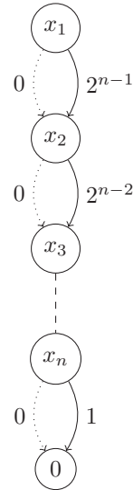
Figure 6: An ordered e\text{-SLDD}_+ representation of f(x_1, \dots, x_n) = \sum_{i=1}^n 2^{n-i} \times x_i .
