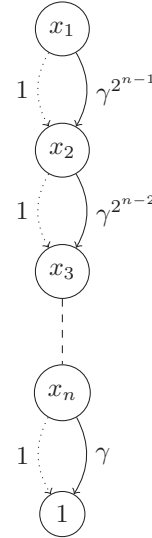
Figure 8: An ordered e\text{-SLDD}_\times representation of f(x_1, \dots, x_n) = \prod_{i=1}^n \gamma^{2^{n-i} \times x_i} .
