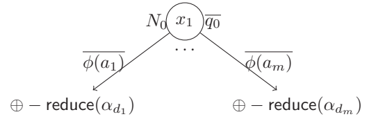
Figure 3: \oplus -reduction of the e-SLDD \alpha .
