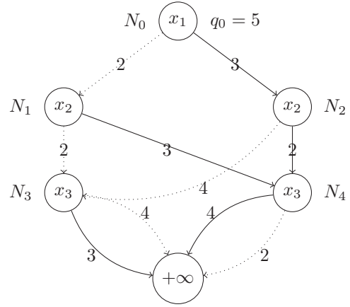
Figure 9: An \text{e-SLDD}_{\min} representation \alpha . The domain of all variables x_1, x_2, x_3 is \{0, 1\} . Every dotted (resp. plain) arc a corresponds to the value v(a) = 0 (resp. v(a) = 1 ).
