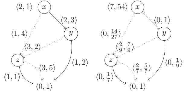
Figure 1: An e\text{-SLDD}_\star formula (left) and the corresponding \min_\star -reduced e\text{-SLDD}_\star formula (right). x, y and z are Boolean variables. A (resp. plain) edge corresponds to the assignment of the variable labeling its source to 0 (resp. 1).
