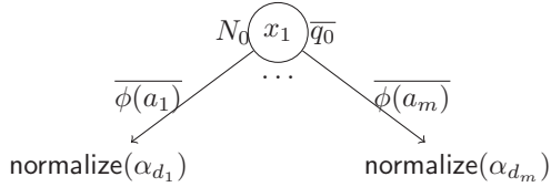
Figure 2: Normalization of an e-SLDD \alpha .
