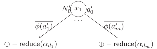
Figure 4: \oplus -reduction of the e-SLDD \alpha' .
