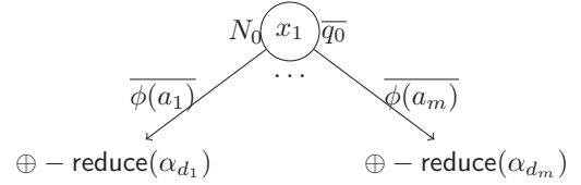
Figure 3: \oplus -reduction of the e-SLDD \alpha .
