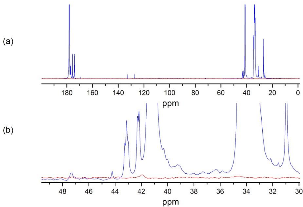
Figure S16: full (a) and partial (b) ^{13}\text{C} NMR spectra of PAA synthesized at 90 °C with thiol and [\text{AA}]_0=2\text{ M} (blue line) and of the contaminated \text{D}_2\text{O} (red line)
