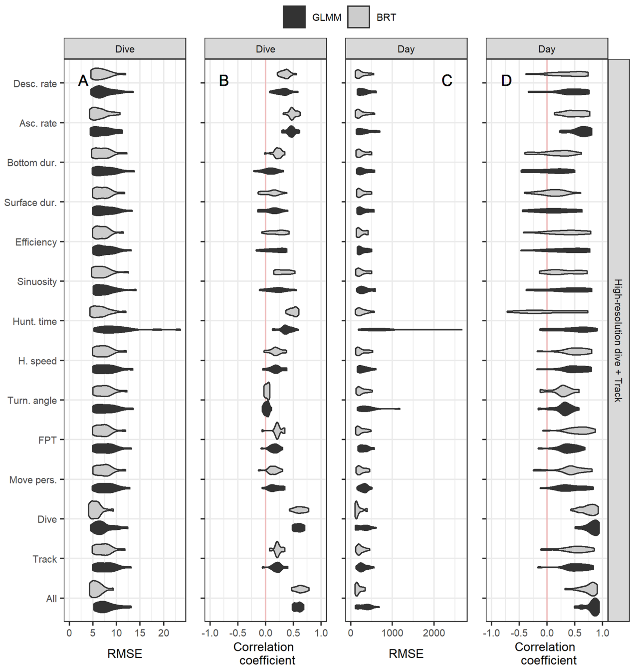
Fig. 5 Performance of each of the models (on the y-axis) in predicting the number of prey encounter events (nPEE) at the scale of dives ( A and B ) and days ( C and D ). Each of the models is fitted with a generalized linear mixed-effect model (GLMM; in black) and with a boosted regression tree (BRT; in grey). The root-mean-square error (RMSE) and the correlation coefficient are computed between the observed values of nPEE for each seal and the predicted values by the model fitted without the focal individual (i.e., leave-one-individual-out cross-validation). The dive model includes all the dive-based metrics, the track model includes all the track-based metrics, and the all model includes all the metrics. Dive metrics are calculated from the high-resolution dive profiles (i.e., at 1 Hz)
