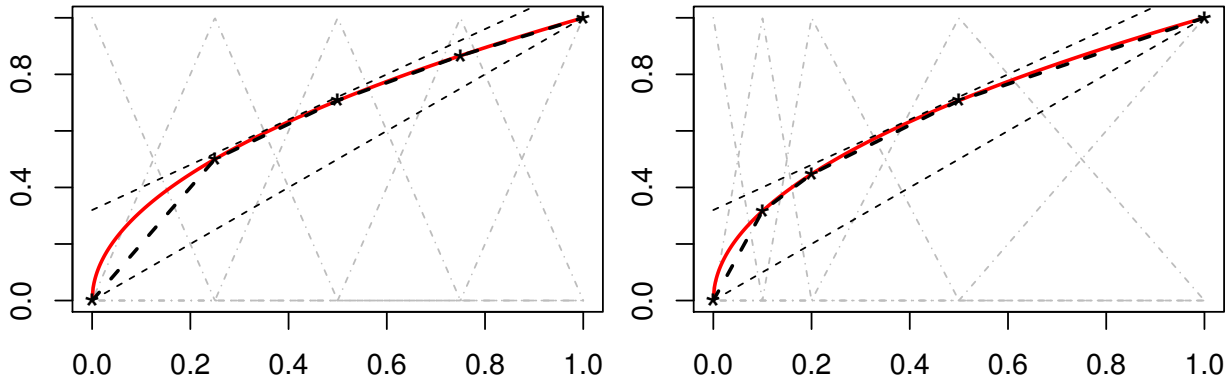
Figure 2: An example of approximating a monotone (nondecreasing) and bounded function f (red solid curve) using a piecewise linear interpolating function \tilde{f}_N (black dashed curve). A uniform (resp. non-uniform) subdivision is used with N = 5 hat functions and knots in the left (resp. right) panel. The gray triangles represent the hat functions, while the black dashed thin lines denote the lower and upper bounds constraints.
