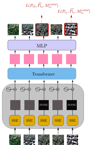
Figure 5. Description of the proposed self-supervised strategy. A percentage M_{rate} of the feature maps encoded by the SSE are masked. U-BARN is trained to reconstruct the previously corrupted patch. The reconstruction loss is computed on the valid pixels, given by the binary mask M^{valid} associated to the masked patch.
