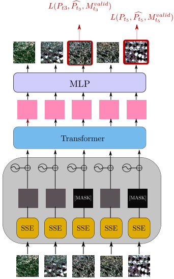
Figure 5. Description of the proposed self-supervised strategy. A percentage M_{rate} of the feature maps encoded by the SSE are masked. U-BARN is trained to reconstruct the previously corrupted patch. The reconstruction loss is computed on the valid pixels, given by the binary mask M^{valid} associated to the masked patch.
