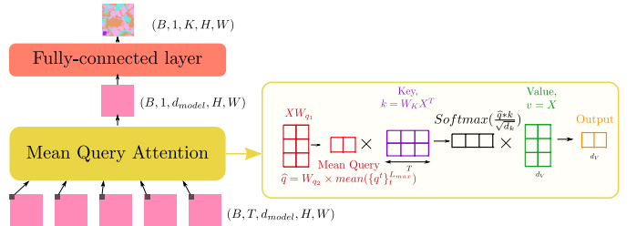
Figure 7. Architecture of the shallow classifier and detailed description of the "mean-query" attention mechanism described in [35]
