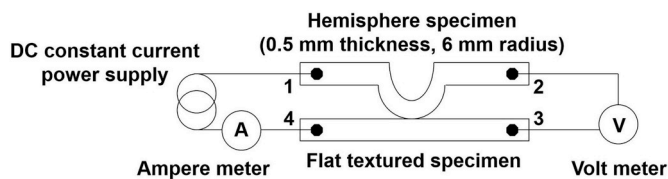
Fig. 6. The geometrical configuration of the hemispherical and flat samples with the four point electrical circuit applied to measure the contact resistance.
