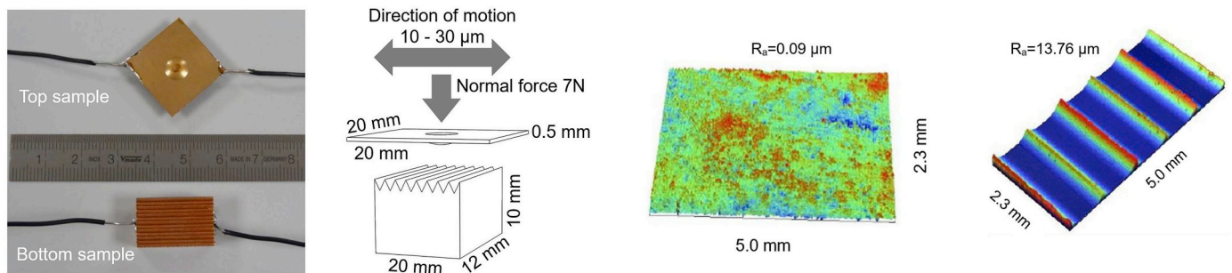
Fig. 3. Left: Surface morphology of a sample polished with 1200 grade sand paper and mirror finished with a diamond paste. Right: milled sample. See Fig. 4 for detailed metrological values.
