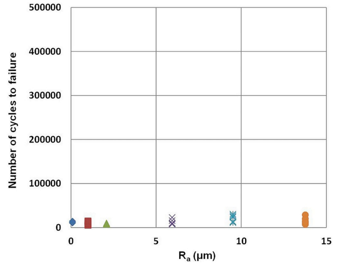
Fig. 10. Number of fretting cycles to failure (100 mΩ failure criterion) as a function of bottom coupon surface roughness. Displacement amplitude applied \pm 30 \mu\text{m} .
