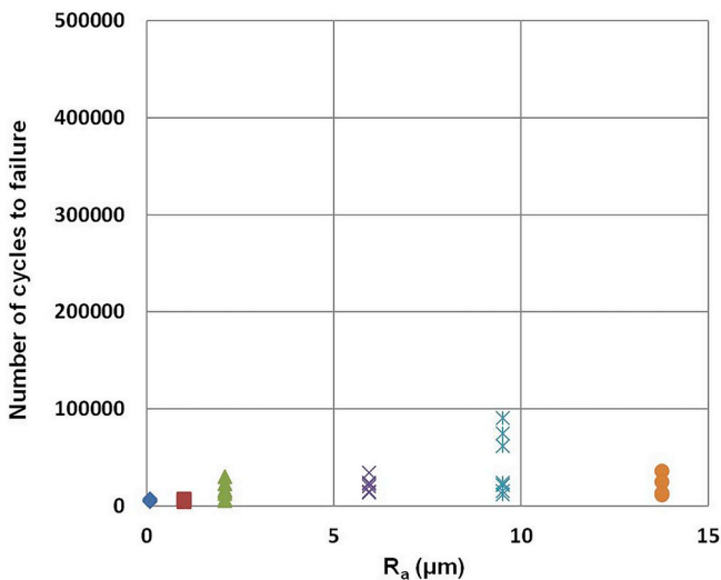
Fig. 9. Number of fretting cycles to failure (100 mΩ failure criterion) as a function of bottom coupon surface roughness. Displacement amplitude applied \pm 20 \mu\text{m} .
