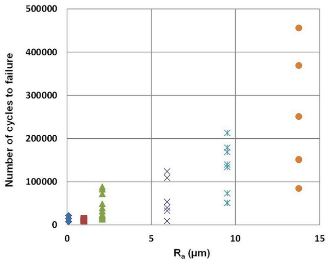
Fig. 8. Number of fretting cycles to failure (100 mΩ failure criterion) as a function of bottom coupon surface roughness. Displacement amplitude applied \pm 10 \mu\text{m} .
