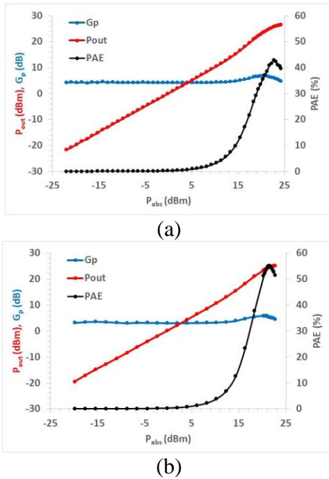
Figure 7: Output power, power gain and power added efficiency versus absorbed power at 40 GHz 2 \times 50 \times 0.075 \mu m^2 AlGaIn/GaN HEMT on Si substrate with non-alloyed ohmic contacts at V_{DS} = 25 V (a) and at V_{DS} = 20 V (b)
