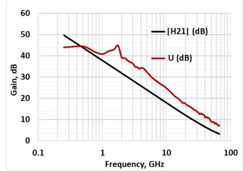
Figure 5: Current gain modulus |H_{21}| , Mason's unilateral gain ( U ) versus frequency for a 2 \times 50 \times 0.075 \mu\text{m}^2 AlGaIn/GaN HEMT on Si substrate with non-alloyed ohmic contacts at V_{GS} = -1.4 V and V_{DS} = 6 V.
