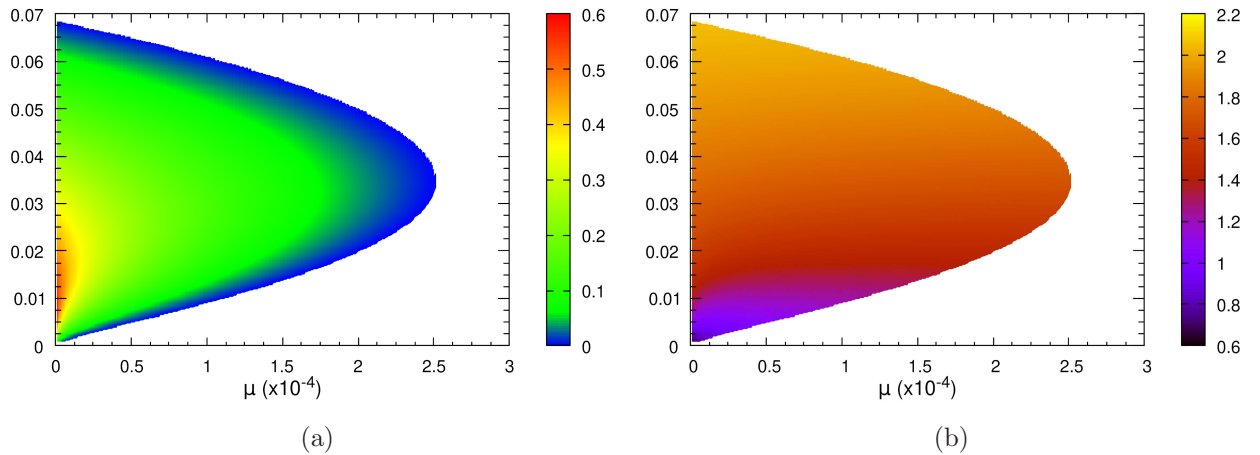
Figure 10: (a) Phase diagram in the plane (\lambda, \mu) , depicting (a) the real part and (b) the imaginary part of the solution of equation (50) for which the real part \text{Re } \Omega (> 0) is the largest.
