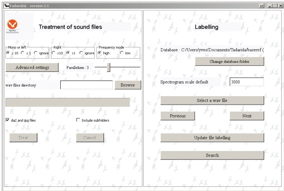
Figure 3: The graphical user interface of Tadarida-L.
