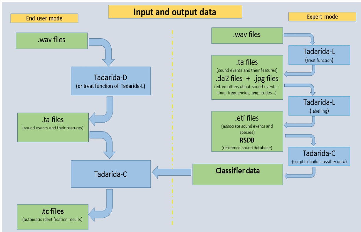
Figure 2: Overview of the data process in both end and expert use modes, detailing input and output file formats of the three modules.
