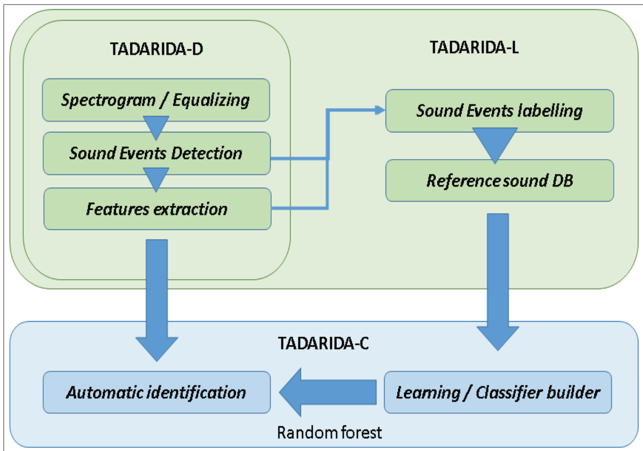
Figure 1: Overview of Tadarida functionalities. Left half corresponds to end use, whereas expert users go through the whole process.
