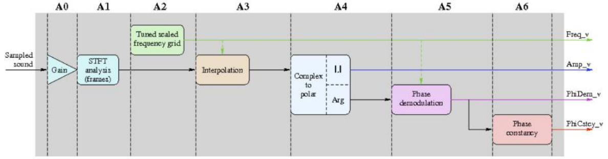
Figure 1. Block diagram of the analysis process of the Snail-Analyser.
