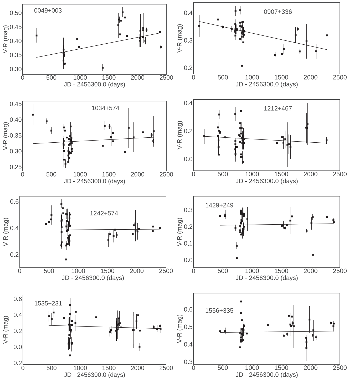
Figure B1. The light curves of colour indices V - R variability during period 2013 April–2019 August of sources: 0049+003, 0907+336, 1034+574, 1212+467, 1242+574, 1429+249, 1535+231, 1556+335, 1607+604, 1612+378, 1722+119, and 1741+597. Details of all sources can be found in Table 5.
