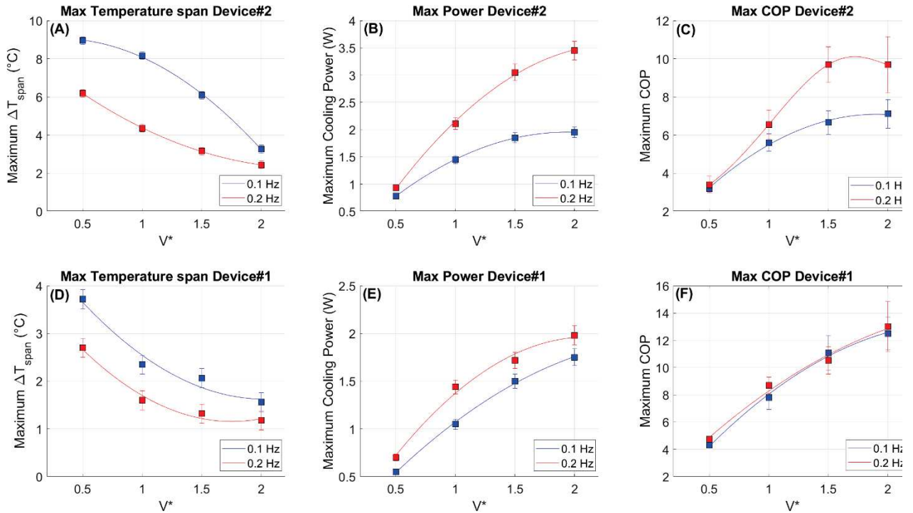
Fig. 7. Summary of the overall performances of the fabricated devices. (A) Maximum values of temperature span vs. V^* , (B) maximum values of cooling power vs. V^* , and (C) maximum COP vs. V^* of Device #2 at 0.1 and 0.2 Hz. (D) Maximum temperature span vs. V^* , (E) maximum values of cooling power vs. V^* , and (F) maximum values of COP vs. V^* of Device #1 at 0.1 and 0.2 Hz.
