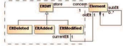
Fig 3. Extract of correspondence meta-model, oriented towards model evolution
