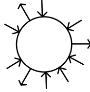
Figure 4.1: A disc of size 3
