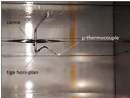
Figure 3 : Canne + micro-thermocouple
