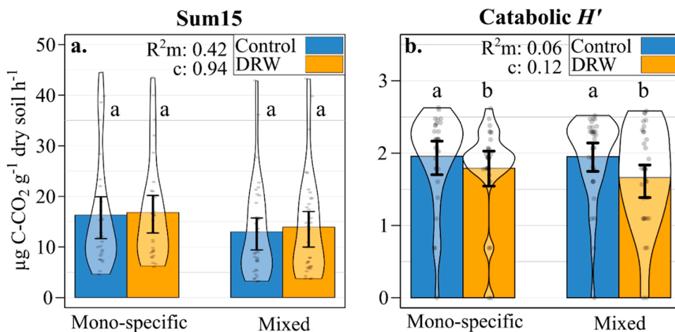
Fig. 5. Microbial catabolic activity a. sum of the microbial catabolic respiration induced by 15 different C-sources (Sum15; \mu\text{g C-CO}_2 \text{ g}^{-1} \text{ dry soil h}^{-1} ), and b. catabolic Shannon diversity index of used substrates ('used' catabolic H' ). Control treatment soils are in blue and DRW treatment soils in orange. Marginal R^2 ( R^2_m ) and conditional ( R^2_c ) values are from LMM results, letters indicate statistically significant differences, and error bars indicate standard error (SE). P-values are coded as: p < 0.05^* , p < 0.01^{**} , p < 0.001^{***} .
