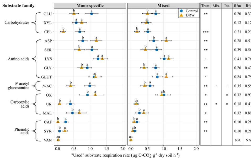
Fig. 6. “Used” respiration rates ( \mu\text{g C-CO}_2 \text{g}^{-1} dry soil \text{h}^{-1} ), i.e. when the respiration was 15 % higher than the respiration without a C addition (i.e. just water added), for the fifteen substrates in soils from mono-specific forest stands (left panel) and mixed tree species stands (right panel) in response to DRW (control in blue and DRW in orange). Abbreviations: D-glucose (GLU), xylan (XYL), cellulose (CEL), N-acetylglucosamine (N-AC), L-asparagine (ASP), L-glutamine (GLUT), L-lysine (LYS), L-serine (SER), L-glycine (GLY), malic acid (MAL), oxalic acid (OX), uric acid (UR), caffeic acid (CAF), syringic acid (SYR), and vanillic acid (VAN). Error bars indicate standard error (SE). Letters indicate statistically significant differences between control and DRW treatments (Treat.) and between tree mixtures (Mix.), and the interaction between the two (Int.) from univariate LMMs for each substrate individually. P-values are coded as: p < 0.05^* , p < 0.01^{**} , p < 0.001^{***} .
