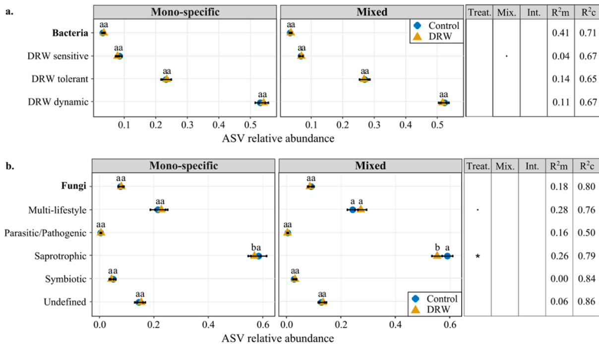
Fig. 2. ASV relative abundance in soils from mono-specific (left panel) and mixed species forest stands (right panel) in response to DRW (control treatment in blue and DRW treatment in orange) for a. bacteria and all subgroups and for b. fungi and all subgroups. Marginal R 2 (R 2 m) and conditional R 2 (R 2 c) values are from LMM results. General bacteria and fungi relative abundances (in bold) are at the genus level, while the subgroups are at the phylum level. Error bars indicate standard error (SE). Letters indicate statistically significant differences and asterisk indicate statistical significance between treatments (Treat.), forest stand type (Mix.), and the interaction between the two (Int.) for each microbial group individually. P-values are coded as: p < 0.05*, p < 0.01**, p < 0.001***.
