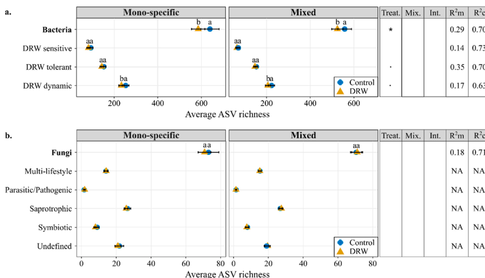
Fig. 1. Average ASV richness in soils from mono-specific (left panel) and mixed species forest stands (right panel) in response to DRW (control treatment in blue and DRW treatment in orange) for a. bacteria and all subgroups and for b. fungi and all subgroups. Marginal R^2 ( R^2m ) and conditional R^2 ( R^2c ) values are from LMM results. Fungal subgroups were not analyzed at the univariate level because PERMANOVA results showed no significant explanatory variable effects at the multivariate level. Error bars indicate standard error (SE). Letters indicate statistically significant differences and asterisk indicate statistical significance between treatments (Treat.), forest stand type (Mix.), and the interaction between the two (Int.) for each microbial group individually. P-values are coded as: p < 0.05^* , p < 0.01^{**} , p < 0.001^{***} .
