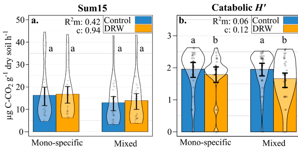
Fig. 5. Microbial catabolic activity a. sum of the microbial catabolic respiration induced by 15 different C-sources (Sum15; \mu\text{g C-CO}_2 \text{g}^{-1} \text{dry soil h}^{-1} ), and b. catabolic Shannon diversity index of used substrates ('used' catabolic H' ). Control treatment soils are in blue and DRW treatment soils in orange. Marginal R^2 ( R^2m ) and conditional ( R^2c ) values are from LMM results, letters indicate statistically significant differences, and error bars indicate standard error (SE). P-values are coded as: p < 0.05^* , p < 0.01^{**} , p < 0.001^{***} .
