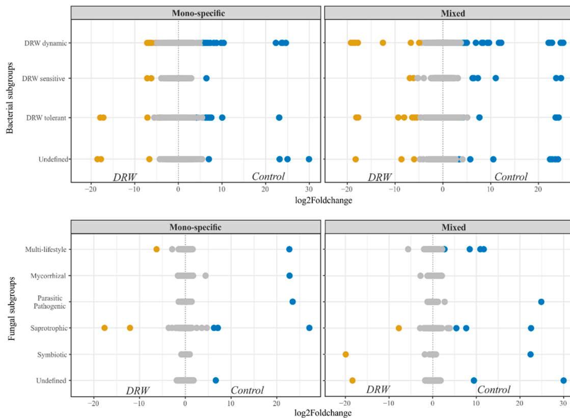
Fig. 4. Differential abundance analysis for bacteria and fungi communities between DRW and control treatments for mono-specific (left panels) and mixed stands (right panels). Gray circles around the zero line represent taxa that are not significantly different in abundance, blue circles represent taxa that are significantly ( p -value < 0.05 ) more abundant in soils from the control treatment (positive relative difference on the right) and yellow circles represent taxa more abundant in soils from the DRW treatment (negative relative difference on the left). See Table S7 –10 for details on differential abundant ASVs.
