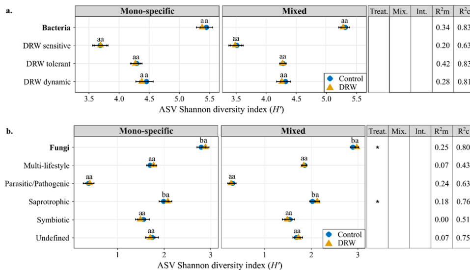
Fig. 3. ASV Shannon diversity index (ASV H') in soils from mono-specific (left panel) and mixed species forest stands (right panel) in response to DRW (control treatment in blue and DRW treatment in orange) for a. bacteria and all subgroups and for b. fungi and all subgroups. Marginal R 2 (R 2 m) and conditional R 2 (R 2 c) values are from LMM results. Error bars indicate standard error (SE). Letters indicate statistically significant differences and asterisk indicate statistical significance between treatments (Treat.), forest stand type (Mix.), and the interaction between the two (Int.) for each microbial group individually. P-values are coded as: p < 0.05*, p < 0.01**, p < 0.001***.
