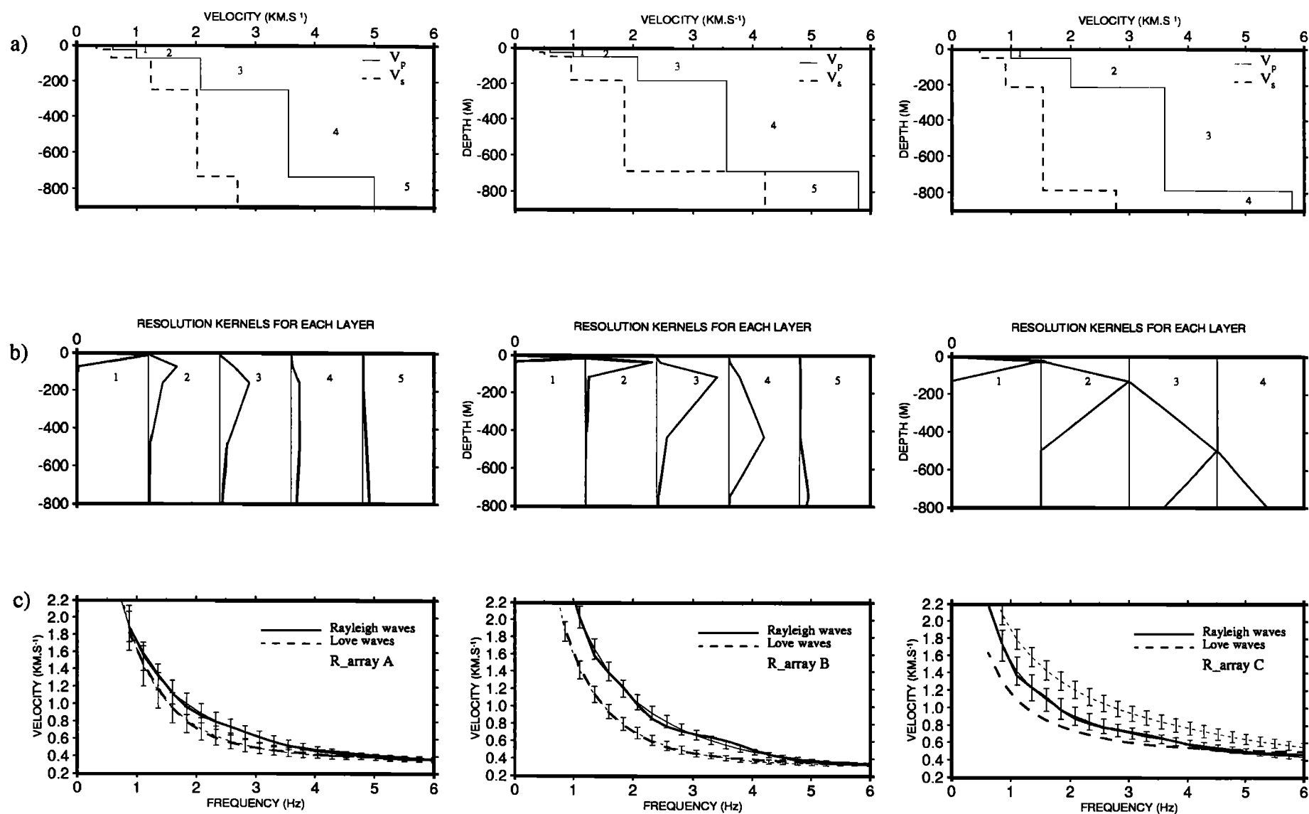
Figure 15. (a) Velocity structures obtained by inversion of the dispersion curves for R_arrays A, B, and C. (b) Resolution kernels for each layer as given by the inversion procedure. (c) Theoretical (thick lines) and observed (thin lines) dispersion curves for Rayleigh (solid lines) and Love (dashed lines) waves.
