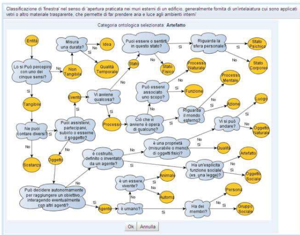
Figure 3. This conceptual map represents the Q/A mechanism underlying TMEO. DOLCE-Spray categories are represented in yellow circles; state transitions are driven by “yes/no” answers (black arrows) to questions enclosed in blue clouds.
