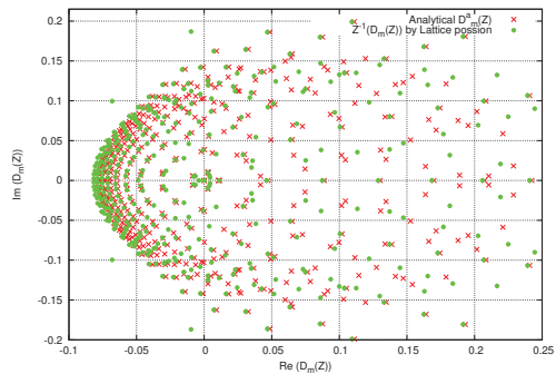
Figure 2: Inversion error for D_m(Z) for n = 5 .
