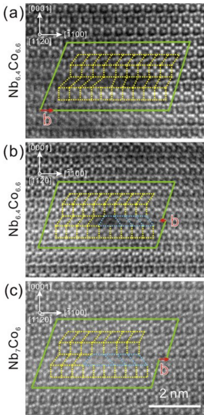
Figure 3. Atomic configurations of the defects on the basal plane of the Nb-Co \mu -phase under an indentation viewed along [1120] axis. HAADF-STEM images of (a) a full dislocation in the \text{Nb}_{6.4}\text{Co}_{6.6} alloy viewed end-on, (b) a partial dislocation bounding a stacking fault in the \text{Nb}_{6.4}\text{Co}_{6.6} alloy, and (c) a partial dislocation bounding a stacking fault in the \text{Nb}_7\text{Co}_6 alloy.
