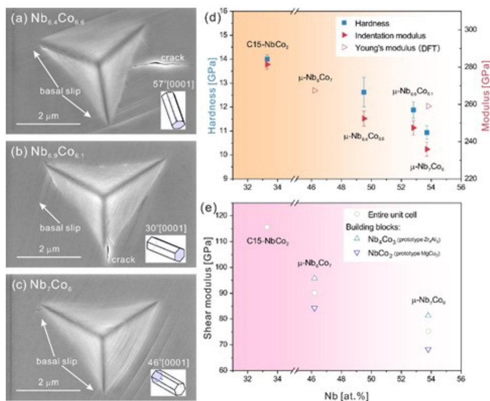
Figure 2. Representative SEM images of indentations of the (a) Nb 6.4 Co 6.6 , (b) Nb 6.9 Co 6.1 and (c) Nb 7 Co 6 alloys showing the surface slip traces after indentation tests. The orientations are denoted by the angle between the loading axis and the c-axis of the Nb-Co \mu -phase. Unit cells representing the orientations are inserted. (d) The composition dependence of hardness and indentation modulus of the Nb-Co \mu -phase measured by nanoindentation tests as well as the Young's modulus determined by DFT (entire unit cell). (e) Calculated basal plane shear moduli of the entire unit cell of C15-NbCo 2 , \mu -Nb 6 Co 7 and \mu -Nb 7 Co 6 and the Nb 4 Co 3 and NbCo 2 building blocks of the two \mu -phases.
