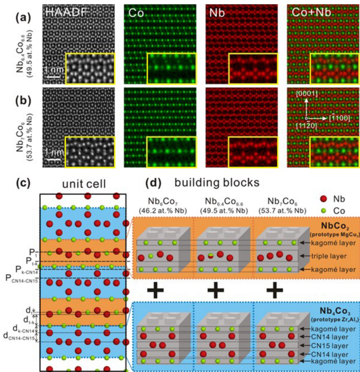
Figure 1. HAADF-STEM images and the corresponding atomic resolution EDS maps of the (a) \text{Nb}_{6.4}\text{Co}_{6.6} and (b) \text{Nb}_7\text{Co}_6 alloys showing the distributions of Co and Nb in the Nb-Co \mu -phase. Schematics of the [11\bar{2}0] projection of the Nb-Co \mu -phase showing the (c) unit cell of \mu\text{-Nb}_6\text{Co}_7 and (d) the stacking of the \text{NbCo}_2 Laves phase and \text{Nb}_4\text{Co}_3 building blocks in \mu\text{-Nb}_6\text{Co}_7 , \mu\text{-Nb}_{6.4}\text{Co}_{6.6} and \mu\text{-Nb}_7\text{Co}_6 . P_t , P_{t-k} , P_{k-CN14} , and P_{CN14-CN15} denote the basal plane between the top and middle layers of the triple layer (the plane between middle and bottom layer is equivalent), the basal plane between the bottom of the triple layer and the kagomé layer, the basal plane between the kagomé layer and the CN14 layer, and the basal plane
