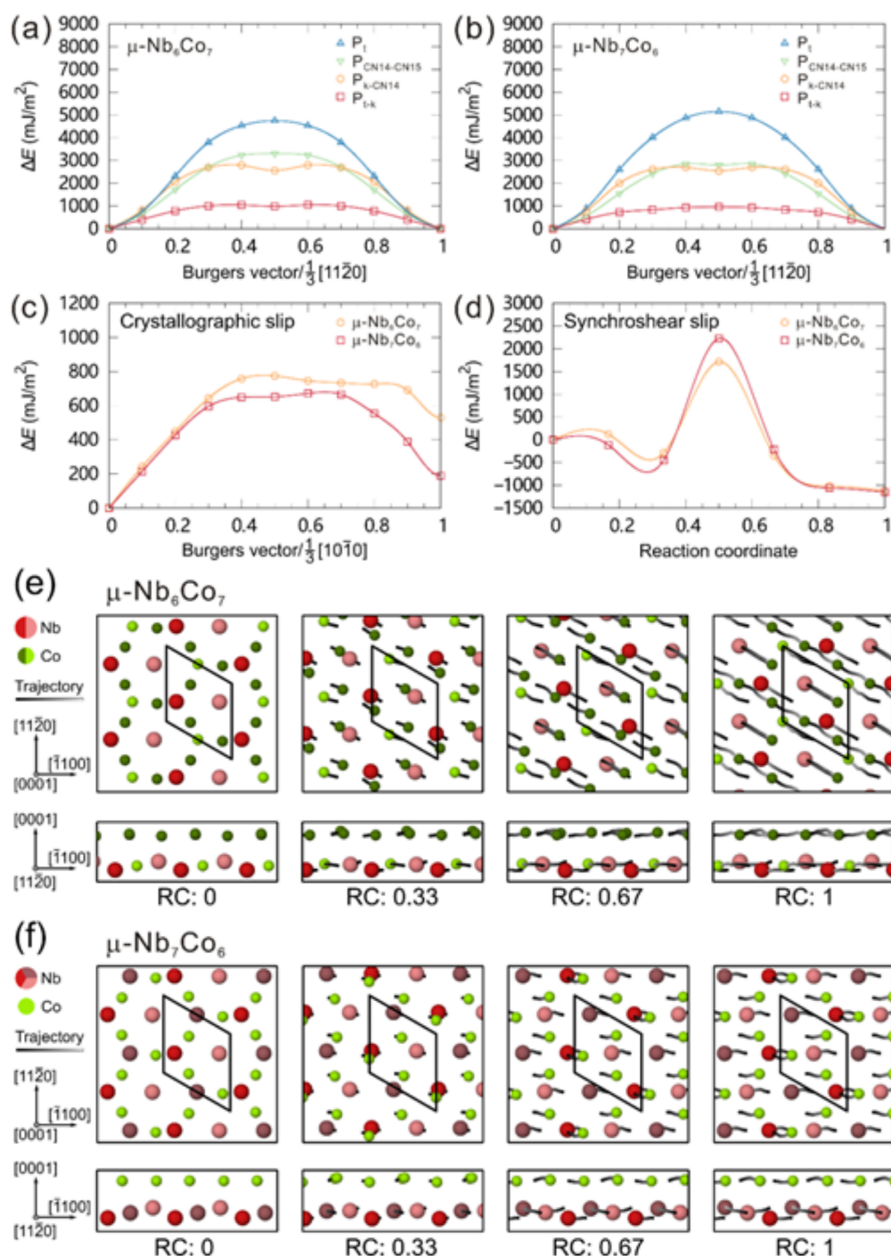
Figure 4. Assessment of the slip mechanisms in \mu -Nb 6 Co 7 and \mu -Nb 7 Co 6 using DFT. GSFE curves of the crystallographic slip along \frac{1}{3}[11\bar{2}0] direction on different basal planes in (a) \mu -Nb 6 Co 7 and (b) \mu -Nb 7 Co 6 . Energy profiles of (c) the crystallographic slip along \frac{1}{3}[10\bar{1}0] direction on P_{t-k} calculated by GSFE and (d) synchroshear calculated using the NEB method.
