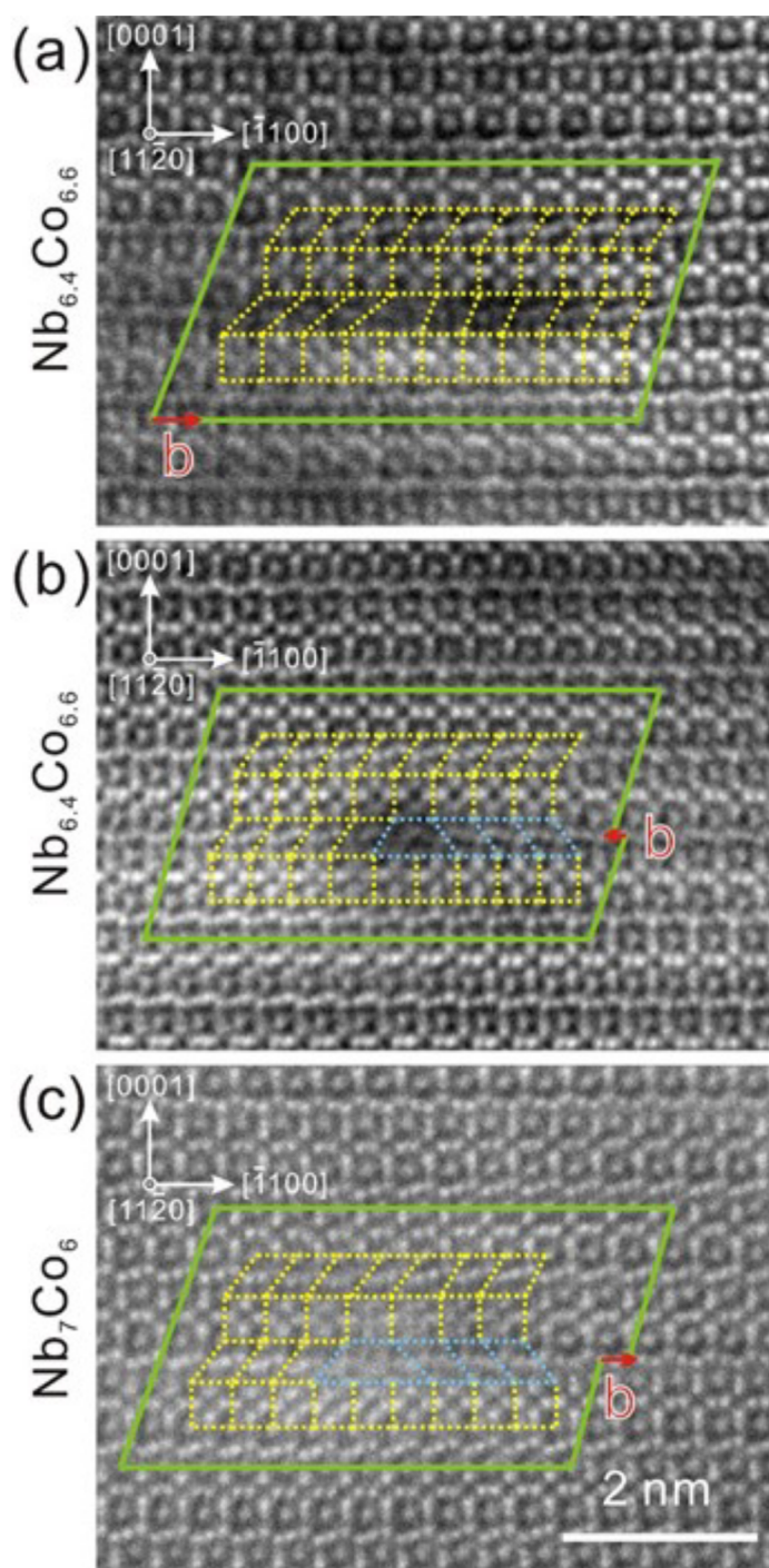
Figure 3. Atomic configurations of the defects on the basal plane of the Nb-Co \mu -phase under an indentation viewed along [11\bar{2}0] axis. HAADF-STEM images of (a) a full dislocation in the \text{Nb}_{6.4}\text{Co}_{6.6} alloy viewed end-on, (b) a partial dislocation bounding a stacking fault in the \text{Nb}_{6.4}\text{Co}_{6.6} alloy, and (c) a partial dislocation bounding a stacking fault in the \text{Nb}_7\text{Co}_6 alloy.
