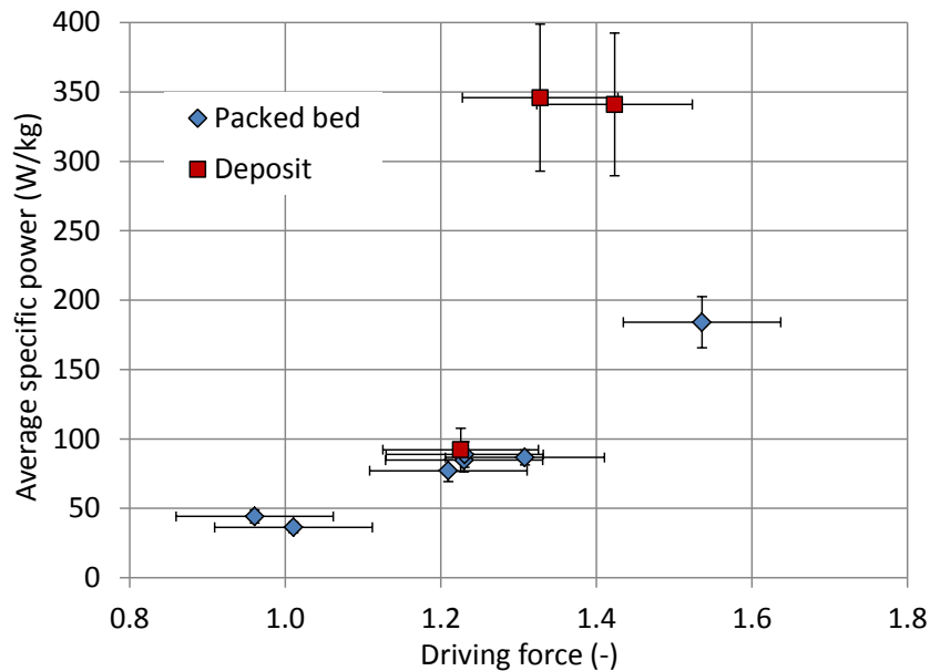
Figure 12: Average specific power vs. driving force for two salt implementations (packed bed and deposit).
