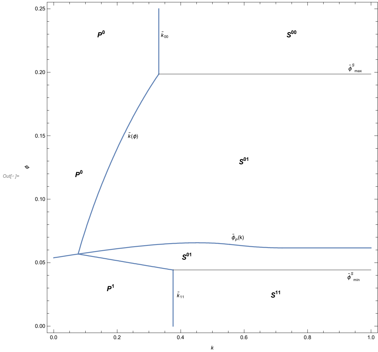
Figure 1 : Separation between P^0 , P^1 , S^{00} , S^{01} and S^{11} contracts in (k, \phi) space
