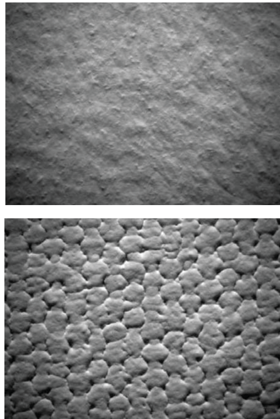
Figure 2. Raking light photomicrographs: Hahnemuhle Fine Art William Turner: Germany, ~2009 (top) and Canson Museum Canvas Water Resistant Matte Canvas: France, April 2008 (bottom).
