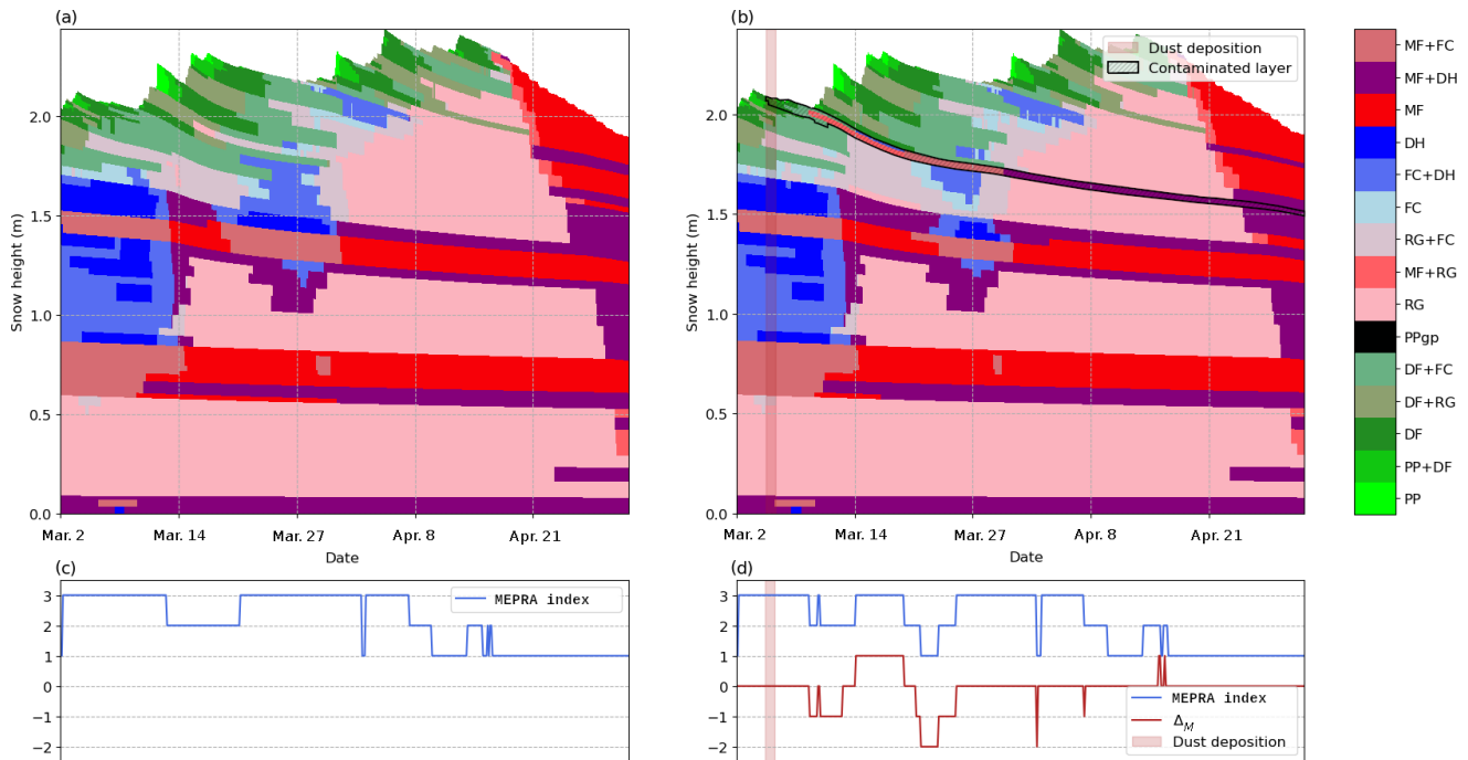
Figure 2. The upper panels show snow profiles for the same member (member 8) of the ensemble simulations on a 40° steep north-facing slope. Panel (a) refers to the no-dust simulation and (b) to the dust simulation. Snow grain shape abbreviations follow the international snow grain shape classification (Fierz et al., 2009) (Table A1), and the shading (hatches) corresponds to the layer contaminated with more than 10^{-4} \text{ g g}^{-1} of dust. The lower panels present the MEPRA stability indicator (in blue) for (c) no-dust and (d) dust simulations. Panel (d) also shows in red the \Delta_M index which represents the difference in stability between simulations.
