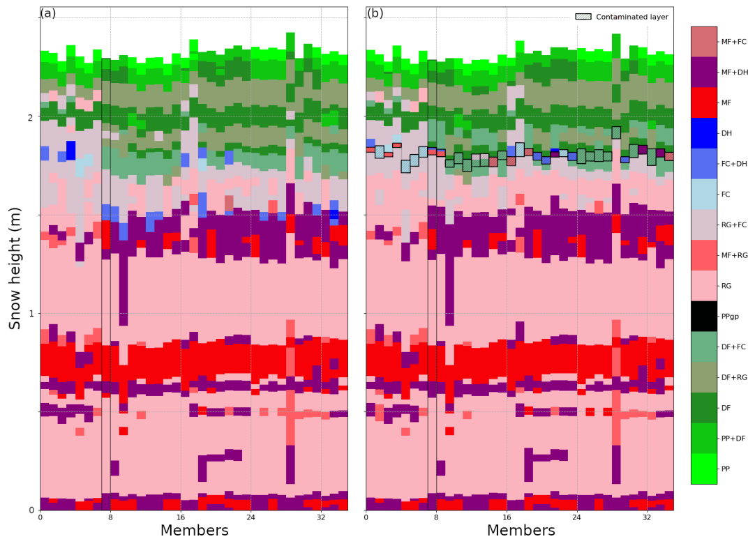
Figure 4. Snow profiles of the 35 members of the no-dust simulation (a) and dust simulation (b) for the northern slope on 18 March 2018 at noon. The member represented in Fig. 2 is surrounded by a black rectangle, and the contaminated layers for each member are hatched in (b). Snow shape names follow the international snow grain shape classification (Fierz et al., 2009).
