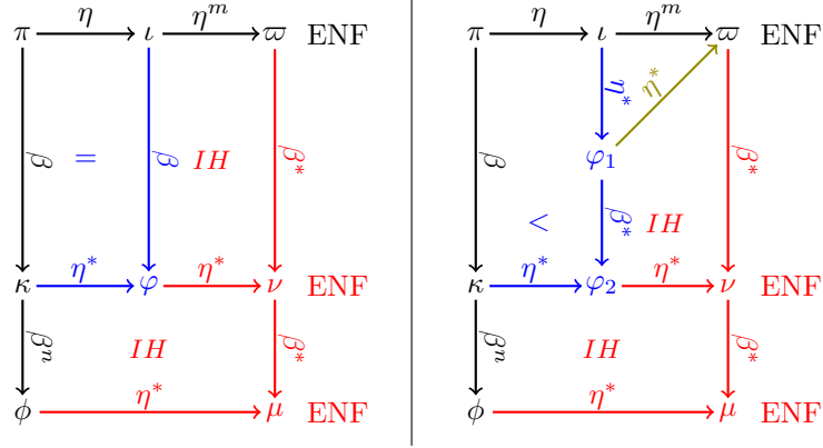
■ Figure 13 Diagrams of the cases of the proof of Lemma 44 (ENF means in \eta -normal form) In blue are uses of Lemma 43, in green of confluence of \xrightarrow{\eta} and in red of the induction hypothesis.
