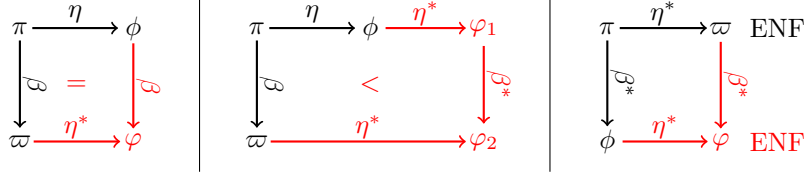
Figure 12 Diagrams of Lemmas 43 (left and center) and 44 (right, ENF means in \eta -normal form)
