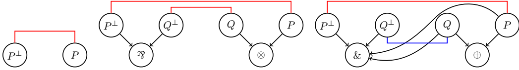
■ Figure 3 Axiom-expansion (from left to right: atoms, \wp \setminus \otimes and \& \setminus \oplus )
