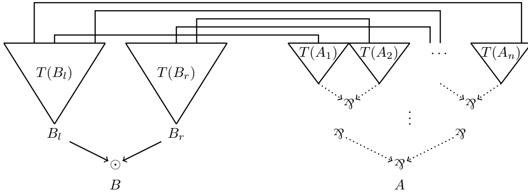
■ Figure 15 Proof-net of Lemma 64 with all terminal \wp -vertices removed
