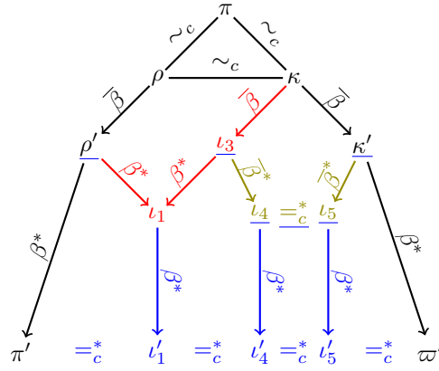
■ Figure 17 Diagram of the case n \neq \emptyset and k = 0 in the proof of Proposition 74
