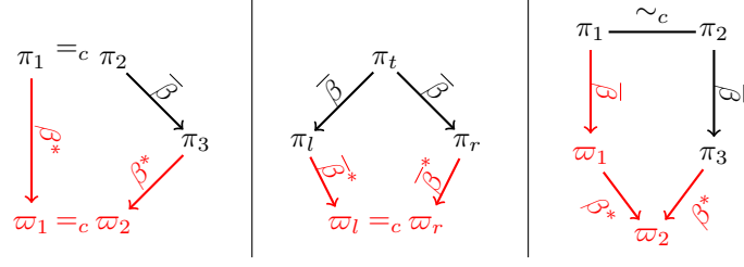
■ Figure 16 Diagrams of Lemmas 71, 72, and 73 (from left to right)
