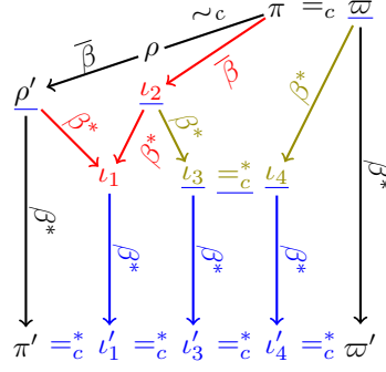
■ Figure 18 Diagram of the case n \neq \emptyset and k = 1 in the proof of Proposition 74
