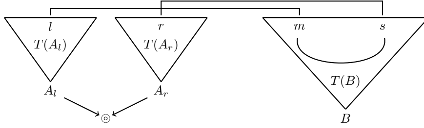
■ Figure 14 Illustration of the proof of Lemma 63
