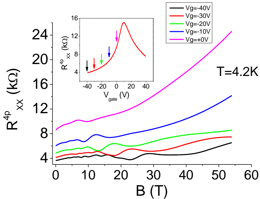
Figure 2: Longitudinal resistance in intermediate disorder few-layer graphene. Measurements are performed at 4.2\text{K} for various carrier densities ( V_{\text{gate}} ). Insert: resistance as a function of the back-gate voltage at zero magnetic field. The colored arrows correspond to the different back gate voltage in the main frame.
