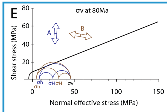
Figure 17 : Mohr diagrams showing the Mohr failure envelope of the Sendji Fm determined from rock mechanics tests and the Mohr circles related to differential stress magnitudes derived from the inversion of calcite twins from each tectonic event, in dry and hydrostatic conditions (see text for details). A, B: Mohr construction for tensor groups E, C, and F related to the far-field Maastrichtian-Paleocene compression between 67 to 60 Ma for dry conditions (A, \sigma_V = 49 MPa) and hydrostatic conditions (B, \sigma_V = 29 MPa). C, D: Mohr construction for tensor groups D and G related to Atlantic ridge push at present-day for dry conditions (C, \sigma_V = 80 MPa) and hydrostatic conditions (D, \sigma_V = 47 MPa). E. Mohr construction for tensor groups A and B related to salt tectonics at 75 Ma in dry conditions ( \sigma_V = 49 MPa.) \sigma_V : vertical principal stress, \sigma_h : minimum horizontal principal stress and \sigma_H : maximum horizontal principal stress.
