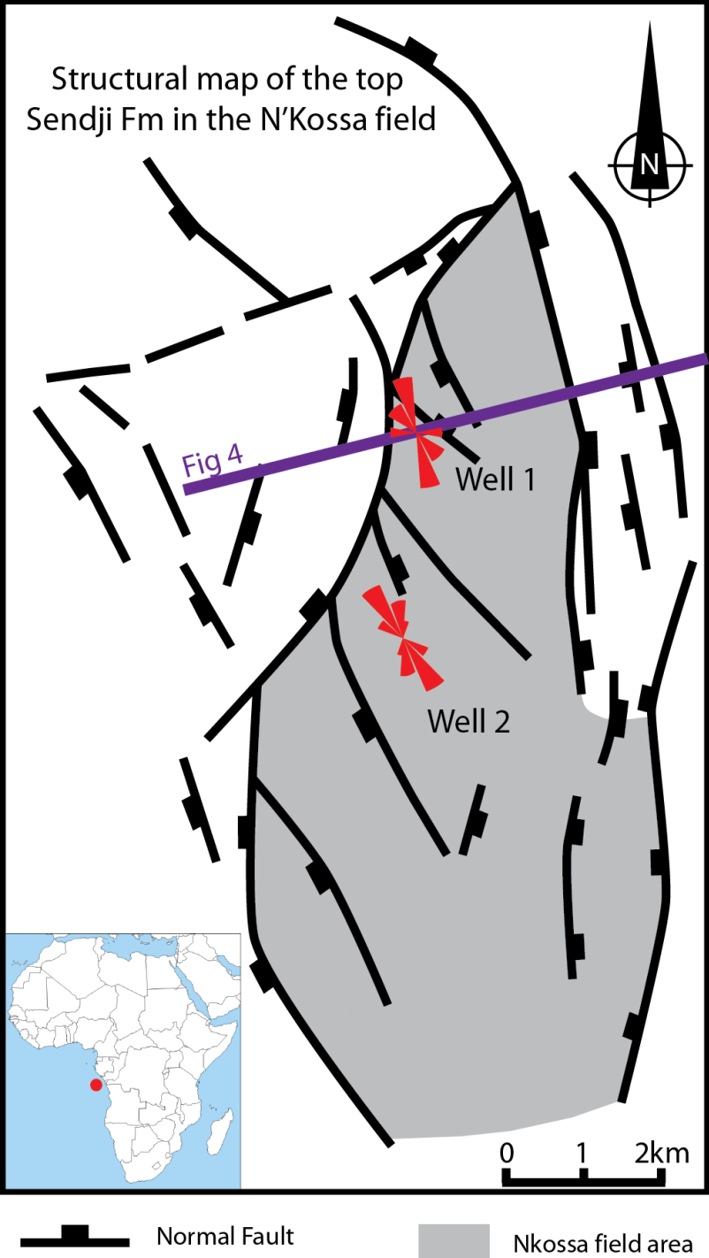
Figure 2 : Structural map of the top of the Sendji Fm in the N'kossa field (modified from TotalEnergies internal report).
