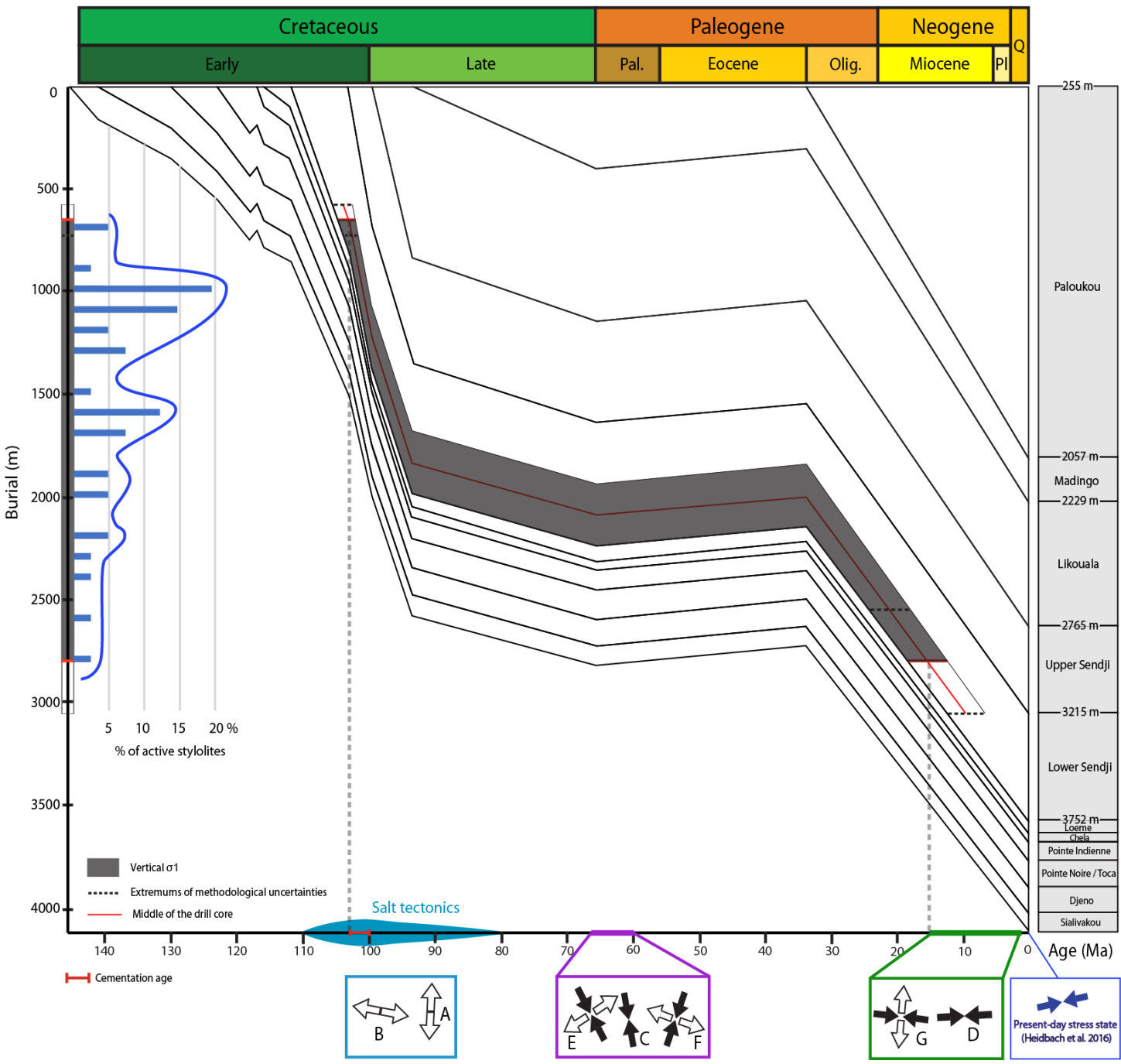
Figure 14 : Burial model of the syn-rift and post-rift formations of the Lower Congo Basin. The results of sedimentary stylolite roughness inversion in terms of depths of active pressure solution results are plotted as a depth histogram. Transitions from vertical to horizontal \sigma_1 periods are illustrated by grey dashed lines (at 101 Ma, 75 Ma, 30 Ma, and 15 Ma) and these estimates are based on the middle of the drill core (indicated by the red line along the burial model). Dark grey areas show periods with vertical \sigma_1 whereas black dashed lines indicate methodological uncertainty limits. The blue area represents the period of active salt tectonics. The average orientation of the horizontal stresses are shown as arrows (with \sigma_1 in black and \sigma_3 in white) in the map view for stress tensors likely coeval with salt tectonics (A and B, blue) possibly related to the intraplate NNW to NNE compressional event during the Maastrichtian-Paleocene times (C, E, and F, purple) and possibly related to the Atlantic ridge push (D and G, green). The present-day stress state is displayed by blue arrows (Heidbach et al. 2016).
