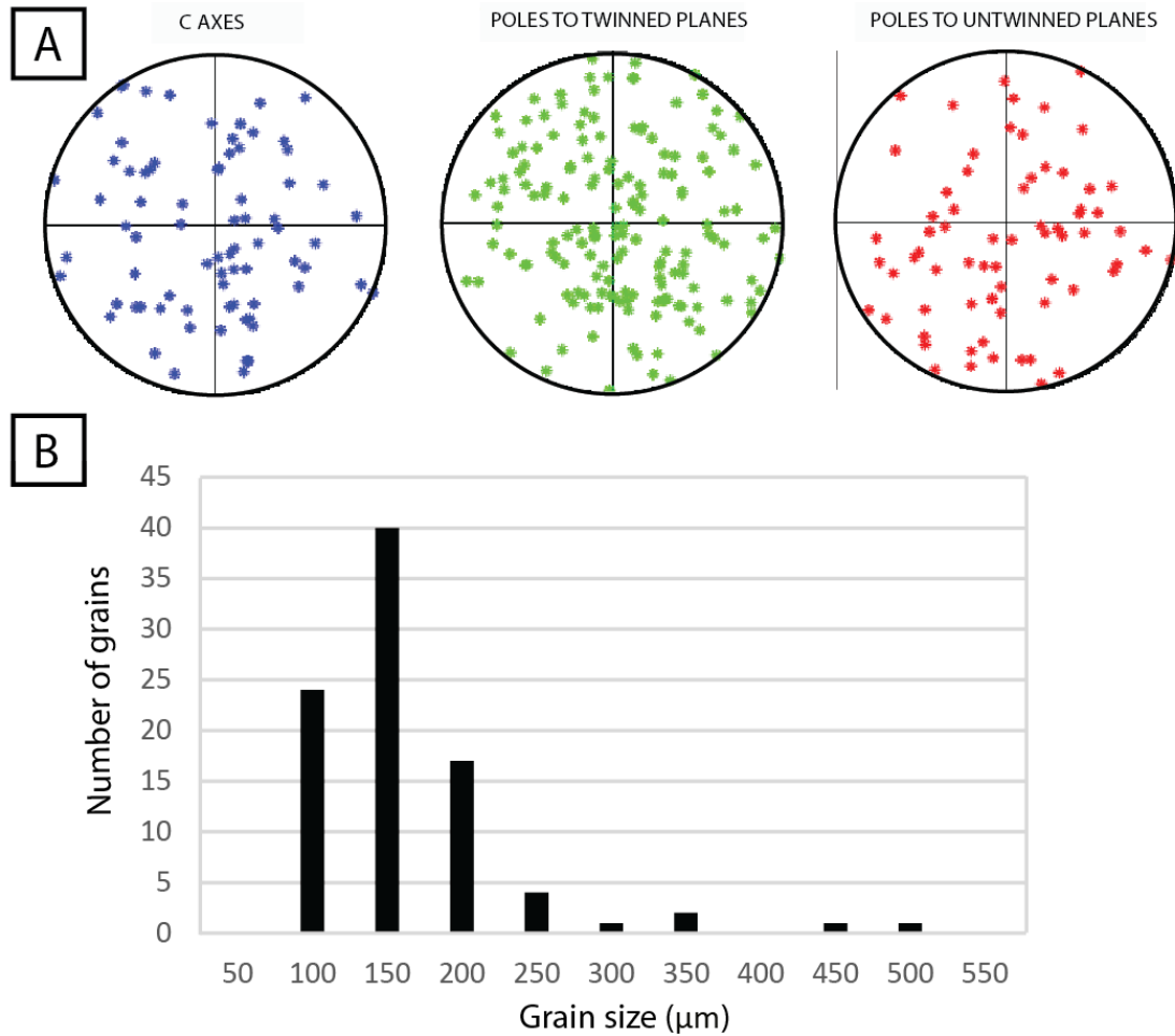
Figure 11 : A. Example of the spatial distribution of optical axes (blue) and poles to twinned (green) and untwinned (red) planes for a sample studied using CSIT-2 (sample 3454.69). B. Example of grain size distribution in the same sample.
