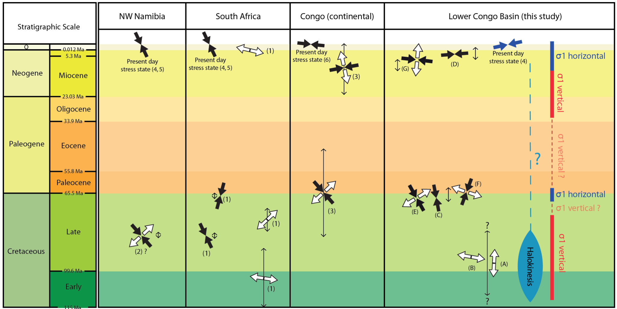
(1) Viola et al. (2012) (3) Nkodia et al. (2020) (5) Viola et al. (2005) (2) Salomon et al. (2015) (4) Heidbach et al. (2016) (6) Delvaux and Bath (2010)
