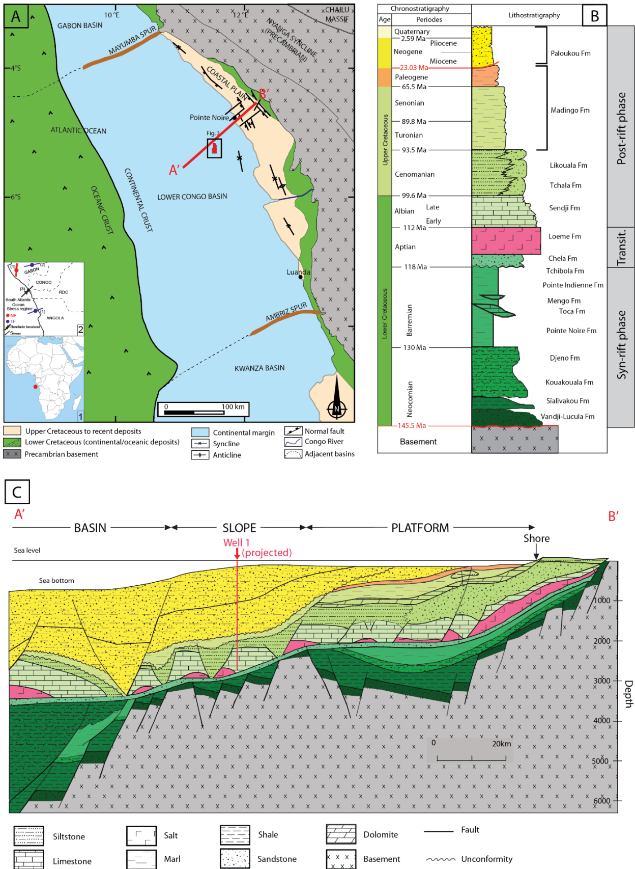
Figure 1 : A. Simplified geological map of the Lower Congo Basin area, offshore Republic of Congo. B. Stratigraphic column of the Lower Congo Basin (modified from TotalEnergies internal report). C. Cross section of the Lower Congo Basin with the horizontal projection of well 1 (modified from Brownfield and Charpentier 2006).
