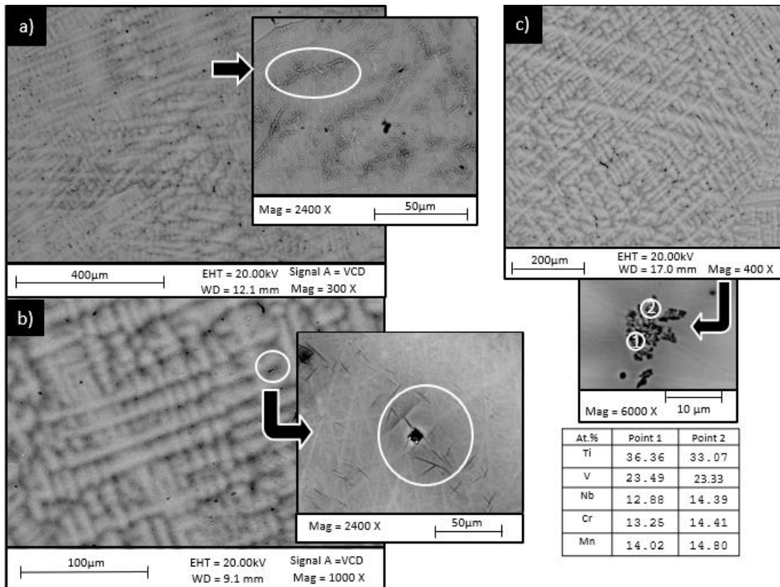
Figure 3 - SEM micrographs of (a) Ti_{35}V_{35}Nb_{20}Cr_5Mn_5 , (b) Ti_{32}V_{32}Nb_{18}Cr_9Mn_9 and (c) Ti_{27.5}V_{27.5}Nb_{20}Cr_{12.5}Mn_{12.5} with the composition of points 1 and 2 indicated in the insert assessed by EDS analyses. Micrographs show the dendritic microstructure, with precipitates in the interdendritic region in detail.
