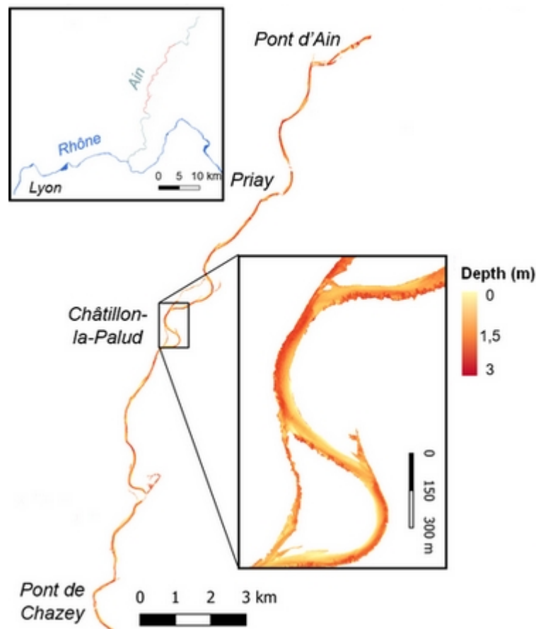
Fig. 1.: Bathymetric map of the Ain River for mean annual flow conditions (127m 3 /s)
