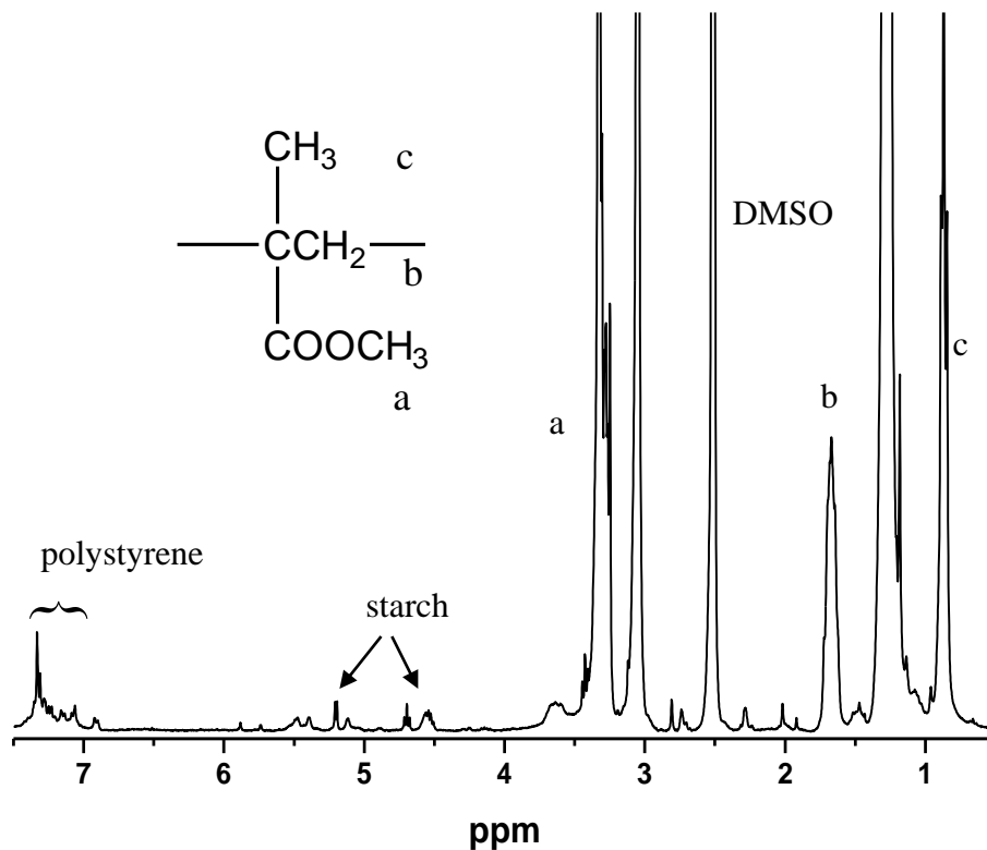
Figure 4: 1 H NMR spectrum of the supernatant of an oligosaccharide grafted onto an MMA swollen polystyrene latex
