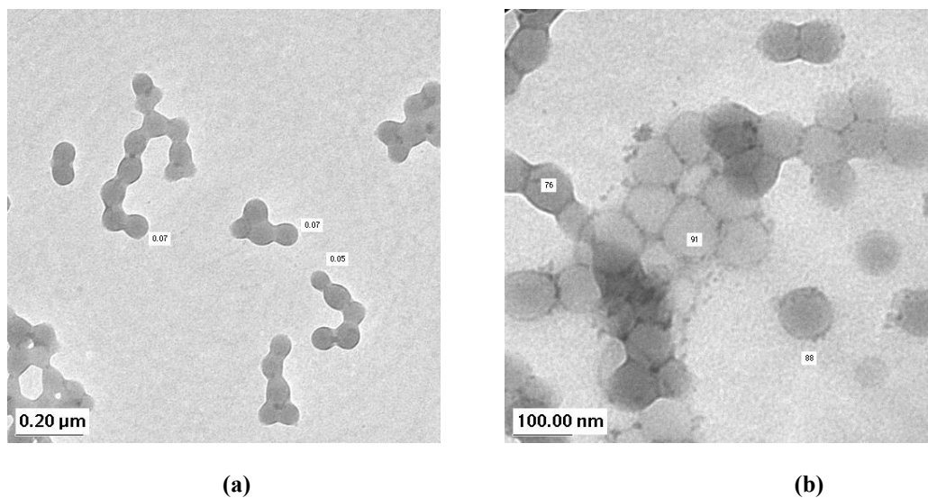
Figure 8: TEM micrographs of (a) PMMA seed latex and (b) oligosaccharide- g -PMMA latex (not dialyzed)
