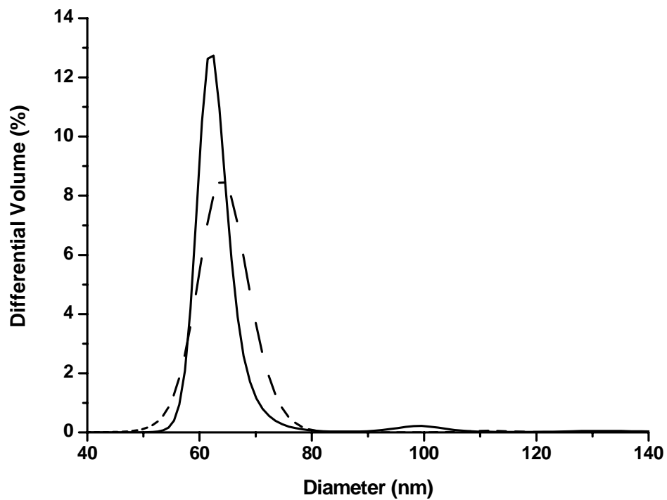
Figure S.2: Hydrodynamic Chromatography Analysis of the cationic polystyrene seed latex (solid line) and the second stage oligosaccharide-g-PMMA/polystyrene latex (dashed line)
