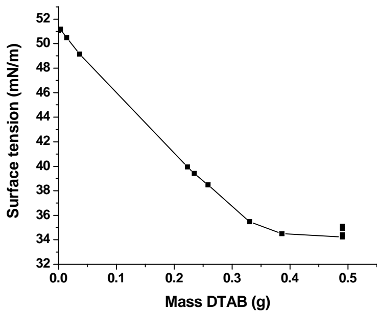
Figure S.4: Surface tension of a cationic polystyrene latex as a function of amount of DTAB
