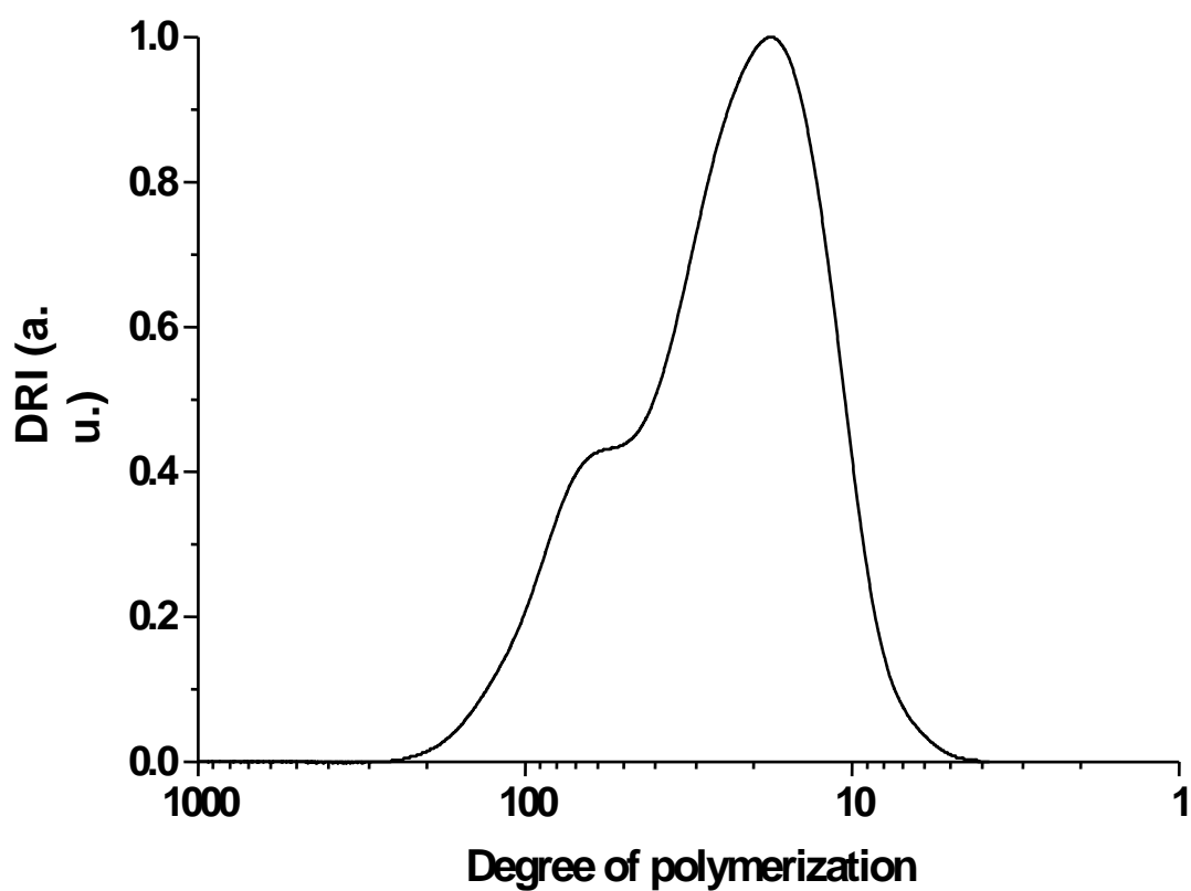
Figure 1: SEC molecular weight distribution of debranched starch. DRI is the raw signal from a Differential Refractive Index detector
