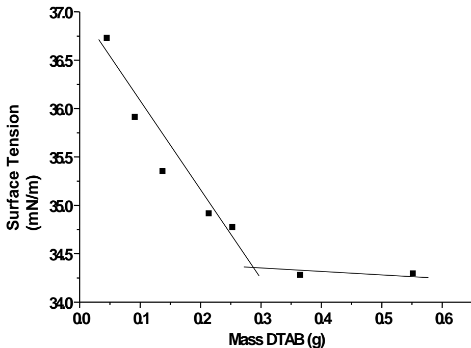
Figure 6: Surface tension measurement for a cationic PMMA latex (40 mL) with increasing additional DTAB. The linear fits on two different ranges are shown as solid lines.
