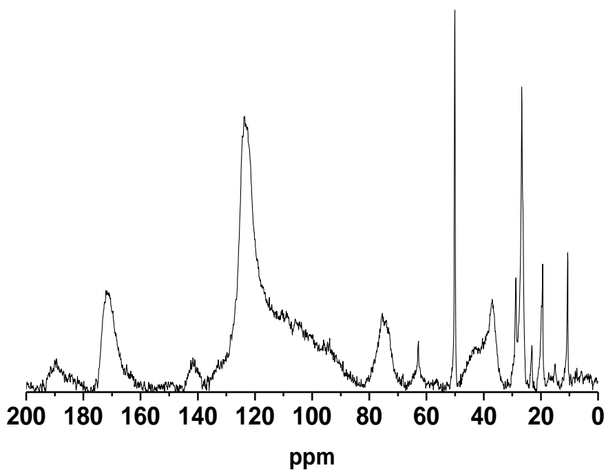
Figure 5: ^{13}\text{C} solid-state NMR spectrum for the precipitate of an oligosaccharide grafted polystyrene/PMMA copolymer
