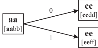
Fig. 1. Construction of the new \widetilde{\text{CRC}} trellis.
