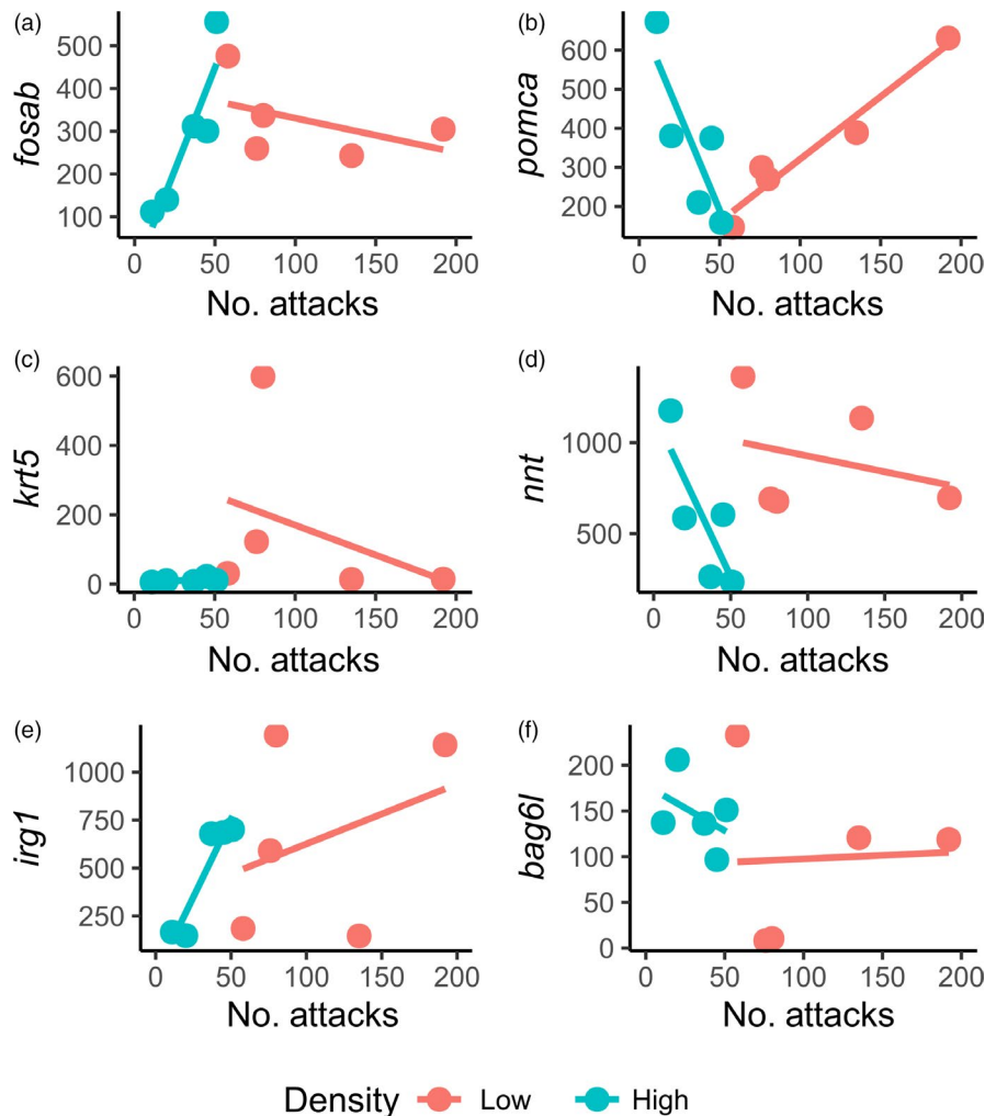
FIGURE 4 Relationship between aggression intensity (no. of agonistic interactions) and gene expression (DESeq2 normalized counts) in the six most aggressive fish at each density. Shown are examples of six responsive genes (out of 19) where there were significant interactions between aggression intensity and rearing density ( q < 0.05 ; Table 1), suggesting that agonistic behaviour is regulated in a density-dependent manner: (a) v-fos FBJ murine osteosarcoma viral oncogene homolog Ab ( fosab ), (b) proopiomelanocortin a ( pomca ), (c) krt5 , (d) nnt , (e) irg1 and (f) bag6l
