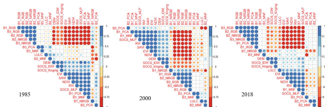
Figure 6: spatial autocorrelations between SOCS and environmental covariates.
