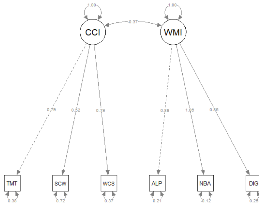
Figure 4. Plot of the SEM model comprising one cognitive control latent index variable (CCI) and another working memory index latent variable (WMI). The dashed line indicates that the loading factors were fixed at a scale of 1.
