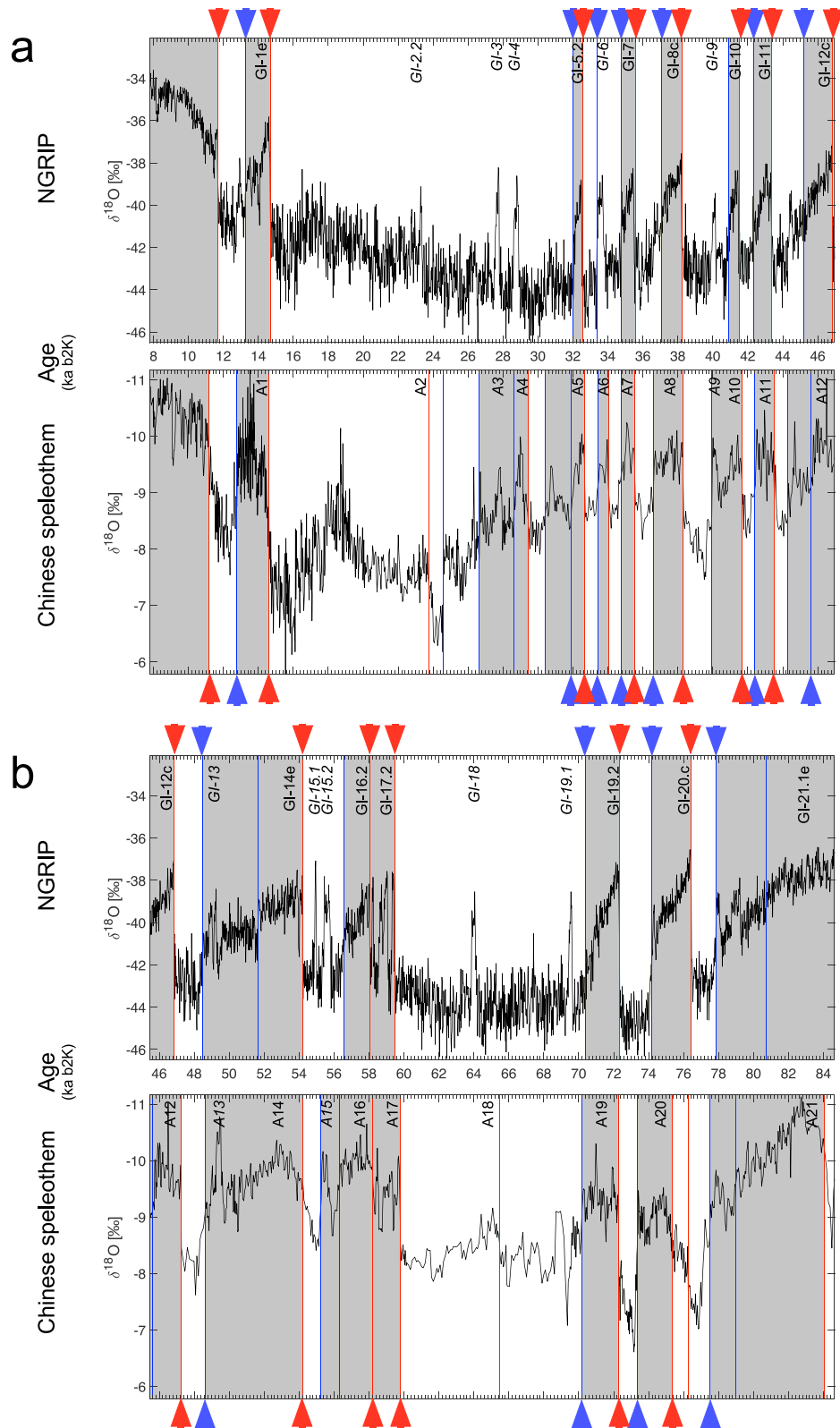
Fig. 1. KS test applied on two high-resolution records, the Greenland NGRIP (Rasmussen et al., 2014) and the Hulu cave (Wang et al., 2001, 2008) \delta^{18}\text{O} records over the past 122 kyr. The records are compared in three panels of 46 kyr each, labeled a, b, and c from youngest to oldest. The grey bars represent interstadials according to Bagniewski et al. (2021), with Greenland interstadials labeled Glx and Chinese interstadials labeled Ax. The red and blue bars indicate abrupt warmings/coolings detected in NGRIP and abrupt moisture increase/drying in the speleothem records, respectively. The red and blue triangles depict the common abrupt warming/moisture and cooling/drying transitions. The NGRIP time scale is in ka b2K while the Hulu time scale is in ka BP. (For interpretation of the references to colour in this figure legend, the reader is referred to the web version of this article.)
