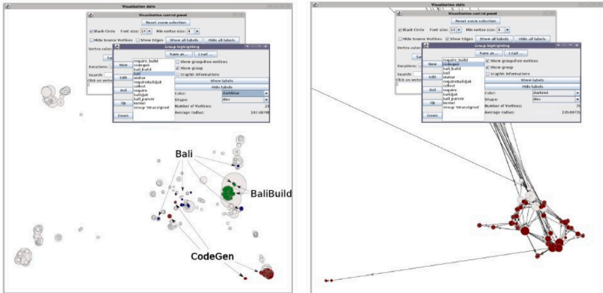
Fig. 6. Transformation. FeatureVisu uses a node-link visualization built on top of a clustering method to depict the feature cohesion metric. For instance, on the left side, we can observe how the implementation elements of the feature BaliBuild (green) are more cohesive than those of the features Bali (blue) and CodeGen (red). On the right side, we can observe an excerpt of the previous layout but this time showing the dependency links between the implementation elements. Figure credits [56]. (For interpretation of the references to color in this figure legend, the reader is referred to the web version of this article.)
