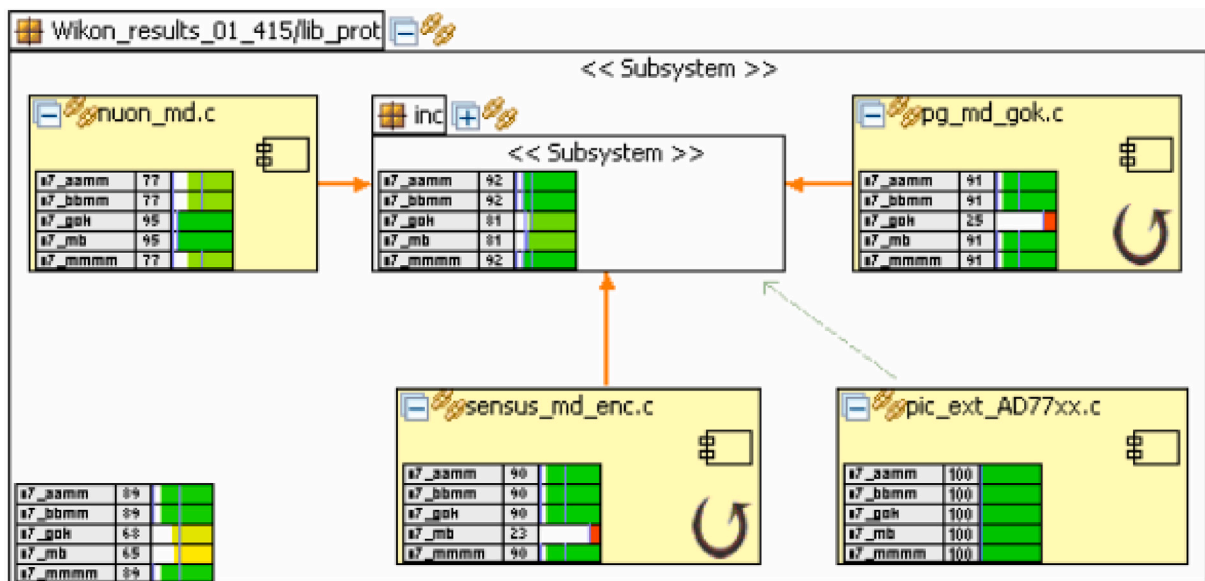
Fig. 5. Architecture Recovery . When it comes to integrating a set of existing similar variants on the way towards an SPL, it is essential to abstract a common architecture. This visualization abstracts from the variants' component architecture to highlight the variance presence. The component diagram depicts which modules are present in several variants (list of names) and to which extent the module is similarly implemented (bar chart). Figure credits [55].
