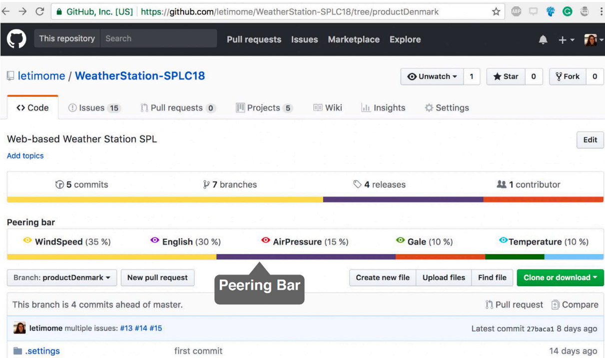
Fig. 2. Variant Integration. PeeringHub mimics GitHub topic bar but now colors denote code churns per feature within a branch. Branches hold temporary developments of variants (e.g., productDenmark ) before being merged back into the Master. In the example, the PeeringBar hints at code efforts being conducted for the variant productDenmark , specifically, for features WindSpeed , English , AirPressure , etc. In this way, if you are upgrading namesake features, you better engage with your productDenmark colleagues to prevent later conflicts during merging. Figure credits [S2]. (For interpretation of the references to color in this figure legend, the reader is referred to the web version of this article.)
