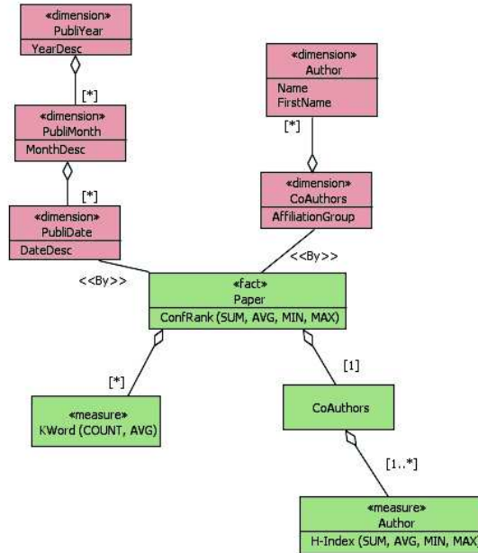
FIG. 7 – Star Class Diagram (StarCD).
