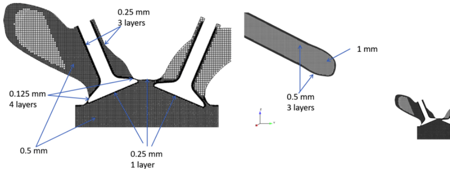
Fig. 11: Mesh topology around the combustion chamber (left) and in the intake port (right) on a cut through the valves at X = 19 mm. No-slip condition applied to refined mesh around valves.
