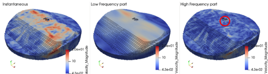
Fig. 8: Application of 3D EMD on the 3D velocity field, local turbulent energy E_k^{HF} (red circle) around spark plug is extracted.
