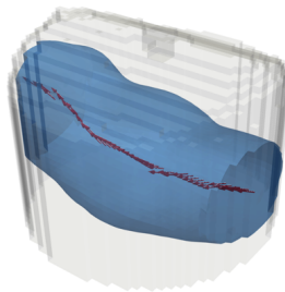
Fig. 20: Tumble vortex core identified by the isosurface of \|\mathbf{\Gamma}_{3p}\| = 0.5 (blue) and tumble center line (red) along X axis around which the tumble motion is organized. Local tumble center at x_0 is of maximal value of \|\mathbf{\Gamma}_{3p}\| for all points at x = x_0 .
