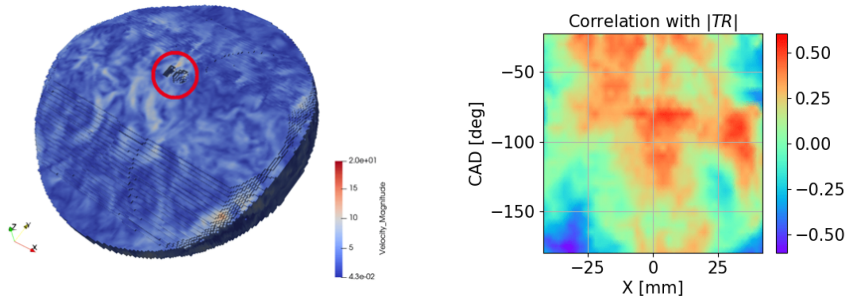
(a) HF part obtained using 3D EMD for 3D velocity field at -22.5 CAD. Evaluation of the averaged local turbulent energy E_k^{HF} (circled in red) around the spark plug.
