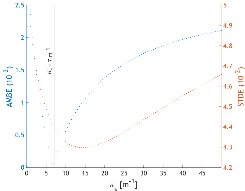
Figure A2. Absolute mean bias error (AMBE, blue) and standard deviation of error (STDE, red) of transmittance ( 10^{-2} ) as a function of \kappa_s ( \text{m}^{-1} ) for dry snow ( N = 168 ) records, considering no surface scattering layer ( i_o = 1 ; h_p = 0 m and \kappa_i = 1 \text{m}^{-1} ). The black line represents the best choice of \kappa_s to minimize AMBE and which gives a reasonable STDE.
