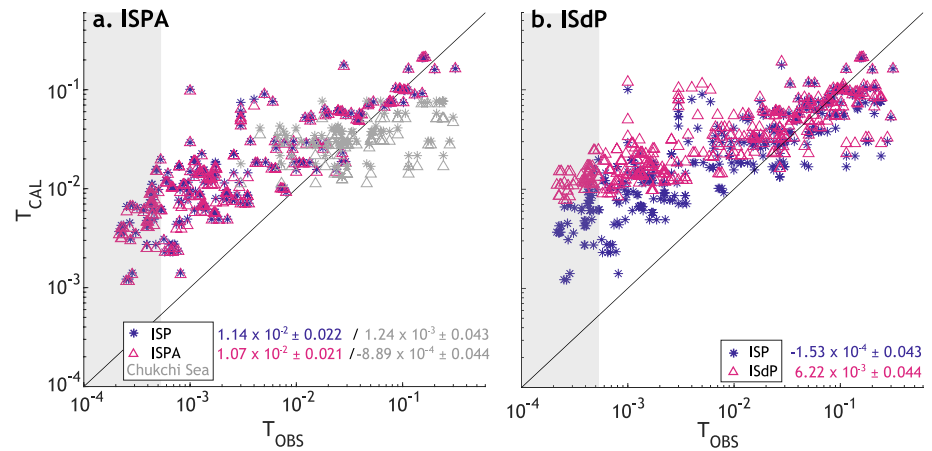
Figure 5. Calculated ( T_{CAL} ) versus observed ( T_{OBS} ) transmittance for the ISPA and ISdP parameterizations. ISPA (a) considers the effects of ice algae. ISdP (b) considers the horizontal distribution of snow depth. In both (a, b) results from ISP are given for reference and numbers at the bottom right corner indicate calculated minus observed transmittance (mean bias error \pm standard deviation). In panel (a), gray symbols depict Chukchi Sea (SUBICE) records; gray numbers correspond to all records with available Chl-a measurements including SUBICE records ( N = 318 ), and colored numbers to the same subset but excluding SUBICE records ( N = 239 ). In panel (b) numbers are computed with the whole data set ( N = 349 ). Gray shading is applied where relative measurement errors on transmittance exceed 50% (see Section 2.1.5).
