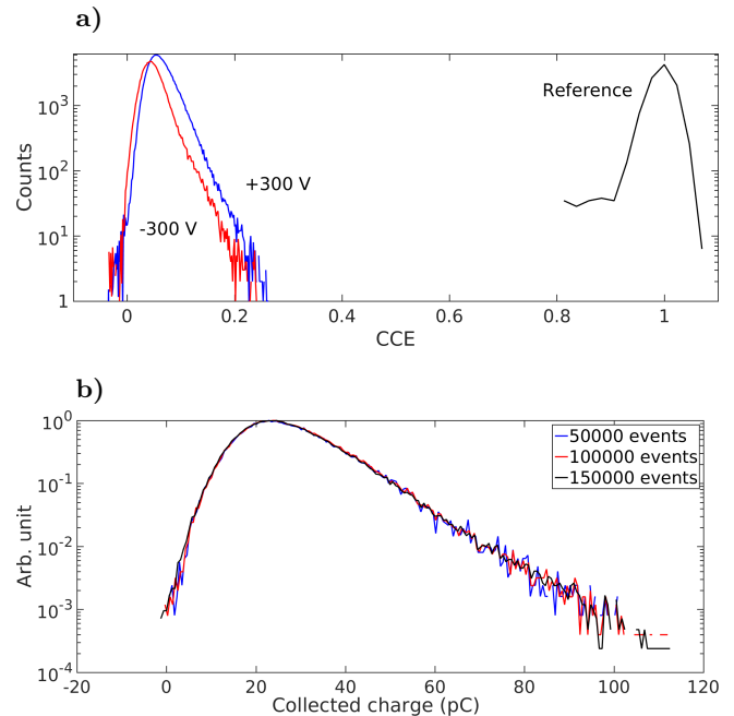
FIG. 4: a): charge collection efficiency (CCE) spectrum for one detector segment (S1) and bias voltages of -300 V and +300 V, normalized to a reference spectrum obtained with a 100 % CCE single crystal CVD diamond detector. b): normalized charge collection spectrum measured after 50000, 100000 and 150000 events, corresponding to roughly 5, 10 and 15 hours of irradiation with the \alpha -particle source.
