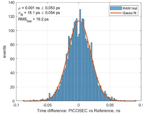
Figure 2. SAT distribution of one channel of the resistive PICOSEC MM. The cathode voltage was set at -490 \text{ V} , the MM mesh at ground and the anode at +290 \text{ V} . The histogram consists of the data after implementing a geometrical cut of a 4 \text{ mm} diameter circle around the pad center to include only fully contained events. A Gaussian fit of the data gives a time resolution of the measured channel of \sigma = 19.2 \text{ ps} .
